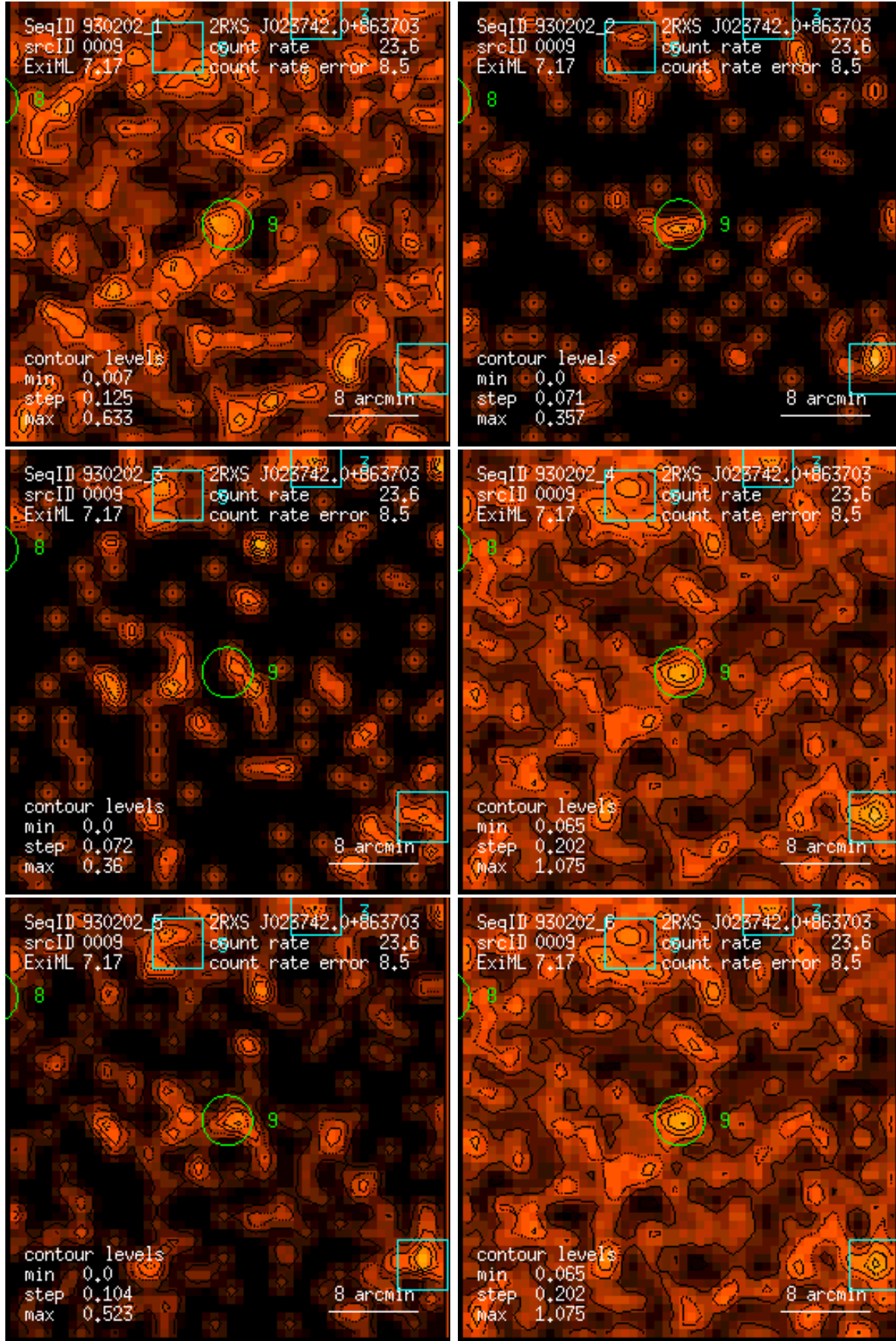
Figure 9: RASS 930202: detection 0009: band rate images, Gaussian filter: (1) PSPC channels 11 – 41, (2) 52 – 90, (3) 91 – 201, (4) 11 – 235, (5) 52 – 201, (6) 11 – 201. Broad band rates in counts/ks. Band rate contour levels in counts/ks/arcmin 2 .
