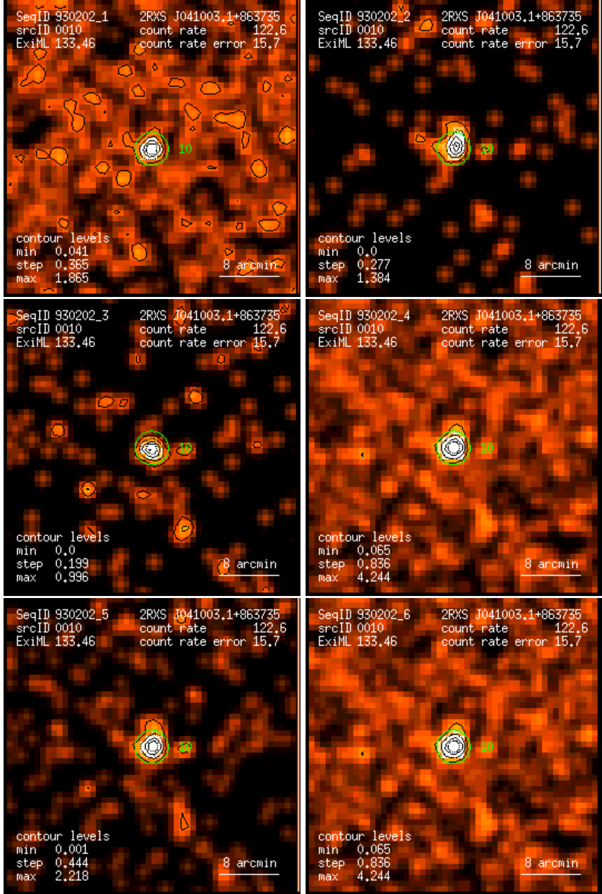
Figure 10: RASS 930202: detection 0010: band rate images, Gaussian filter: (1) PSPC channels 11 – 41, (2) 52 – 90, (3) 91 – 201, (4) 11 – 235, (5) 52 – 201, (6) 11 – 201. Broad band rates in counts/ks. Band rate contour levels in counts/ks/arcmin 2 .
