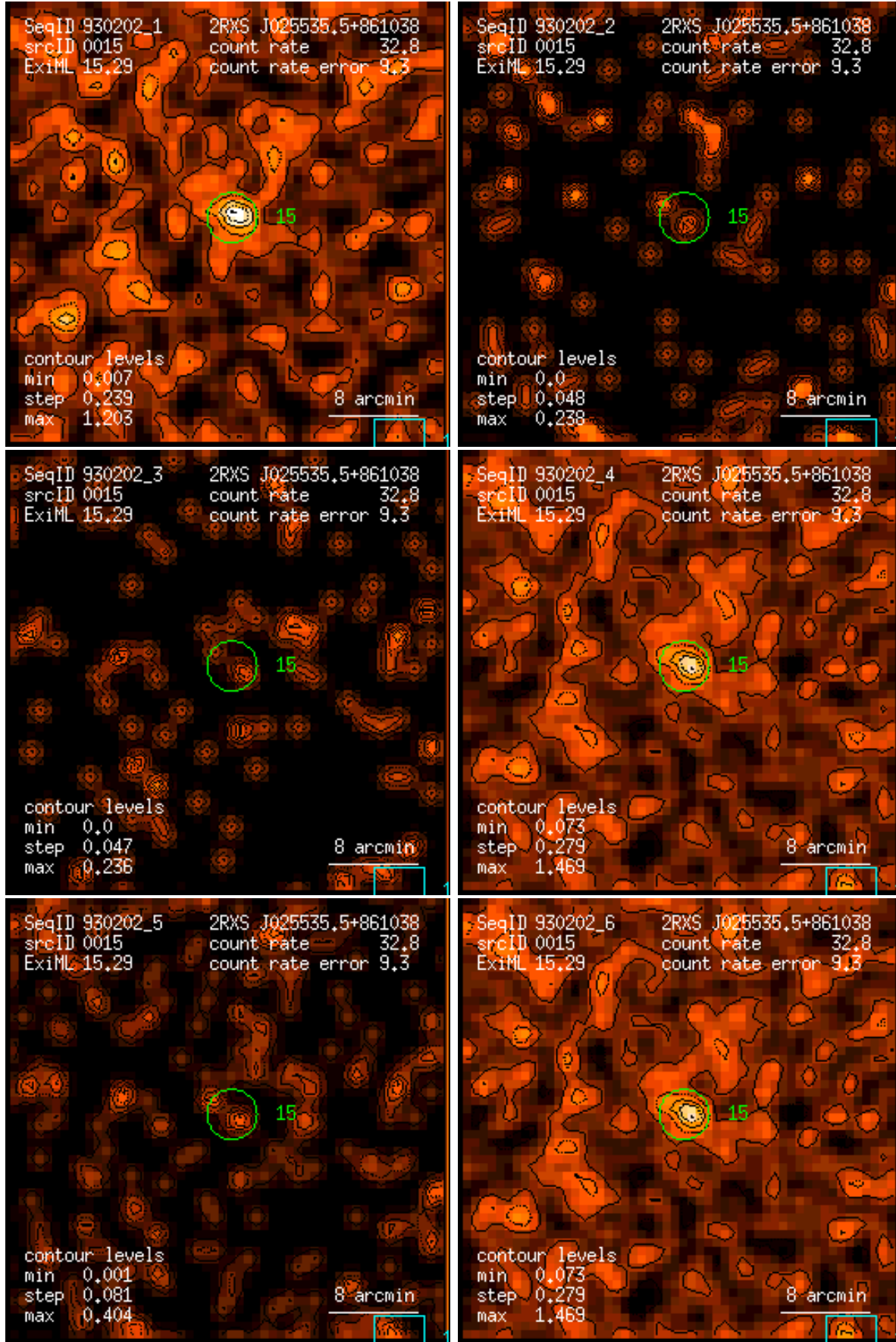
Figure 15: RASS 930202: detection 0015: band rate images, Gaussian filter: (1) PSPC channels 11 – 41, (2) 52 – 90, (3) 91 – 201, (4) 11 – 235, (5) 52 – 201, (6) 11 – 201. Broad band rates in counts/ks. Band rate contour levels in counts/ks/arcmin 2 .
