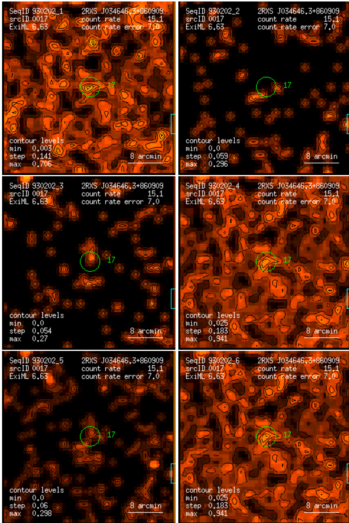
Figure 17: RASS 930202: detection 0017: band rate images, Gaussian filter: (1) PSPC channels 11 – 41, (2) 52 – 90, (3) 91 – 201, (4) 11 – 235, (5) 52 – 201, (6) 11 – 201. Broad band rates in counts/ks. Band rate contour levels in counts/ks/arcmin 2 .
