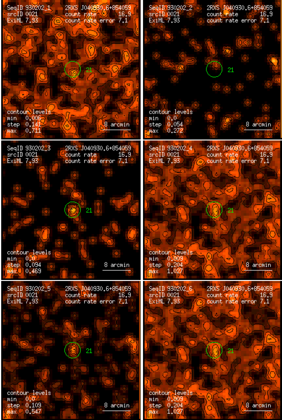
Figure 21: RASS 930202: detection 0021: band rate images, Gaussian filter: (1) PSPC channels 11 – 41, (2) 52 – 90, (3) 91 – 201, (4) 11 – 235, (5) 52 – 201, (6) 11 – 201. Broad band rates in counts/ks. Band rate contour levels in counts/ks/arcmin 2 .
