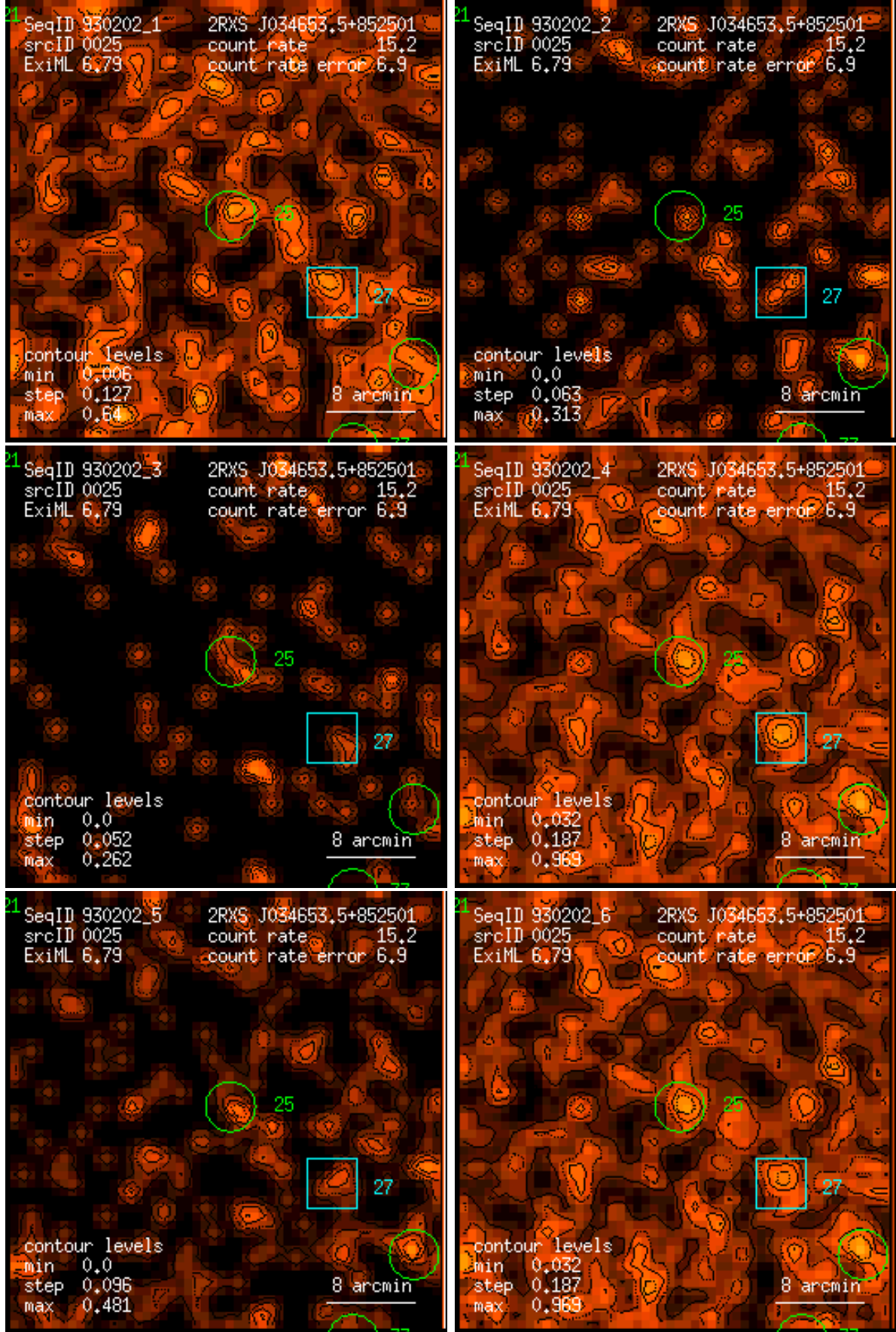
Figure 25: RASS 930202: detection 0025: band rate images, Gaussian filter: (1) PSPC channels 11 – 41, (2) 52 – 90, (3) 91 – 201, (4) 11 – 235, (5) 52 – 201, (6) 11 – 201. Broad band rates in counts/ks. Band rate contour levels in counts/ks/arcmin 2 .
