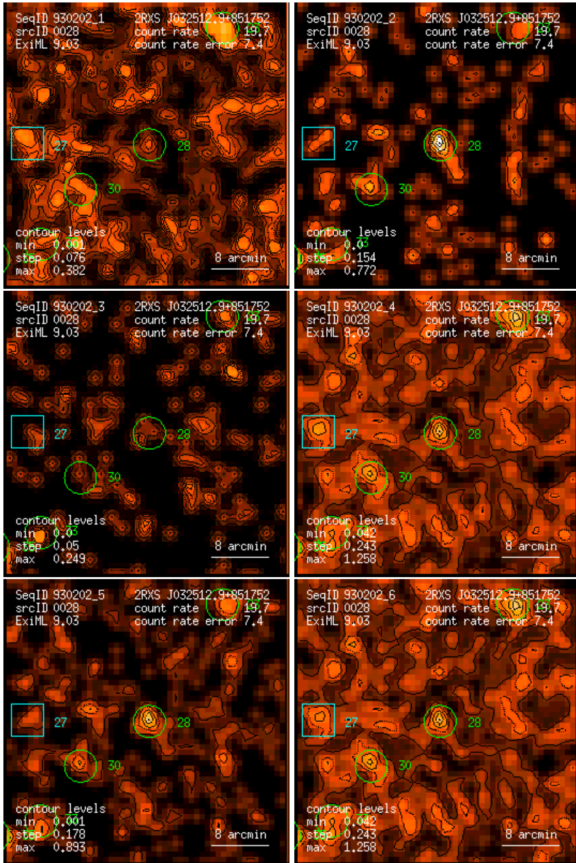
Figure 28: RASS 930202: detection 0028: band rate images, Gaussian filter: (1) PSPC channels 11 – 41, (2) 52 – 90, (3) 91 – 201, (4) 11 – 235, (5) 52 – 201, (6) 11 – 201. Broad band rates in counts/ks. Band rate contour levels in counts/ks/arcmin 2 .
