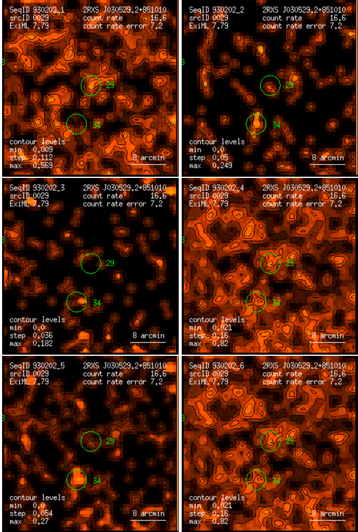
Figure 29: RASS 930202: detection 0029: band rate images, Gaussian filter: (1) PSPC channels 11 – 41, (2) 52 – 90, (3) 91 – 201, (4) 11 – 235, (5) 52 – 201, (6) 11 – 201. Broad band rates in counts/ks. Band rate contour levels in counts/ks/arcmin 2 .
