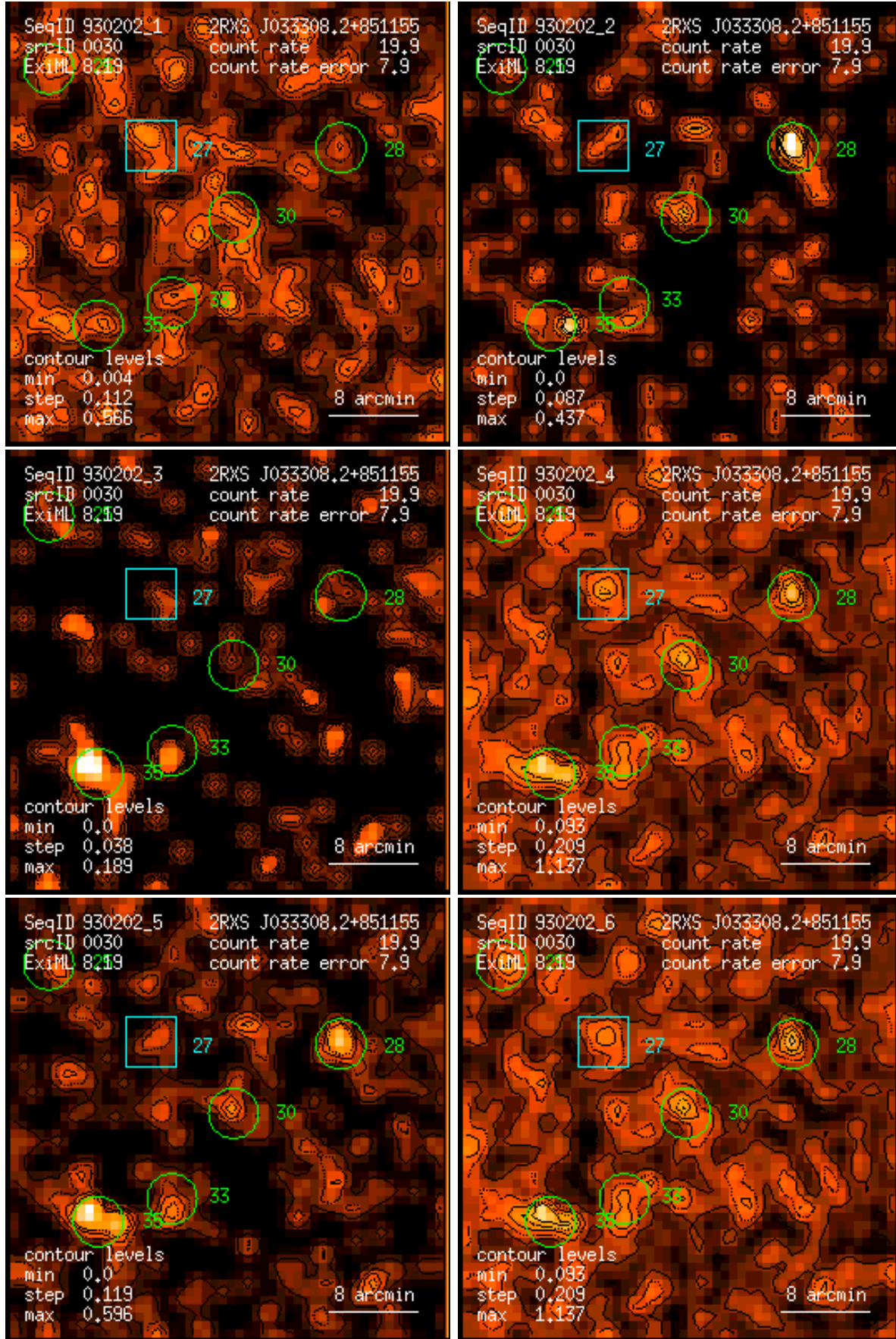
Figure 30: RASS 930202: detection 0030: band rate images, Gaussian filter: (1) PSPC channels 11 – 41, (2) 52 – 90, (3) 91 – 201, (4) 11 – 235, (5) 52 – 201, (6) 11 – 201. Broad band rates in counts/ks. Band rate contour levels in counts/ks/arcmin 2 .
