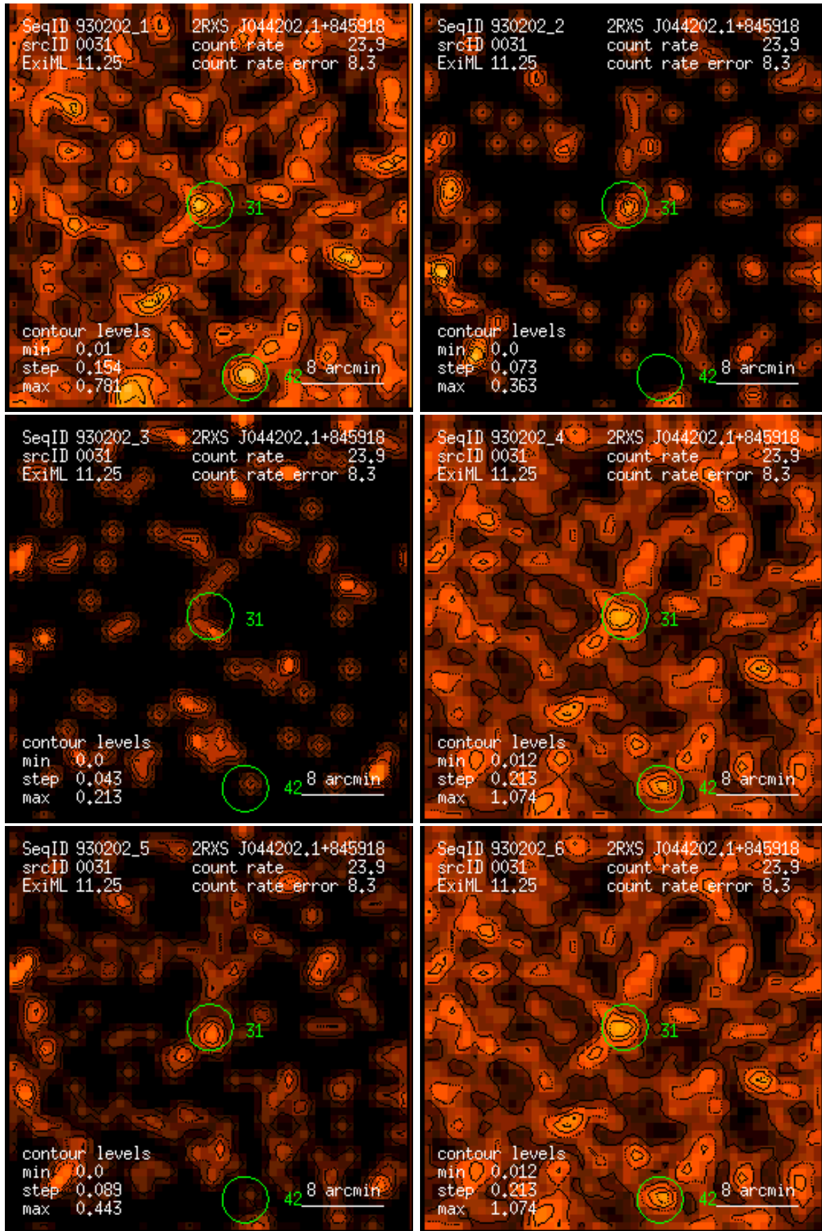
Figure 31: RASS 930202: detection 0031: band rate images, Gaussian filter: (1) PSPC channels 11 – 41, (2) 52 – 90, (3) 91 – 201, (4) 11 – 235, (5) 52 – 201, (6) 11 – 201. Broad band rates in counts/ks. Band rate contour levels in counts/ks/arcmin 2 .
