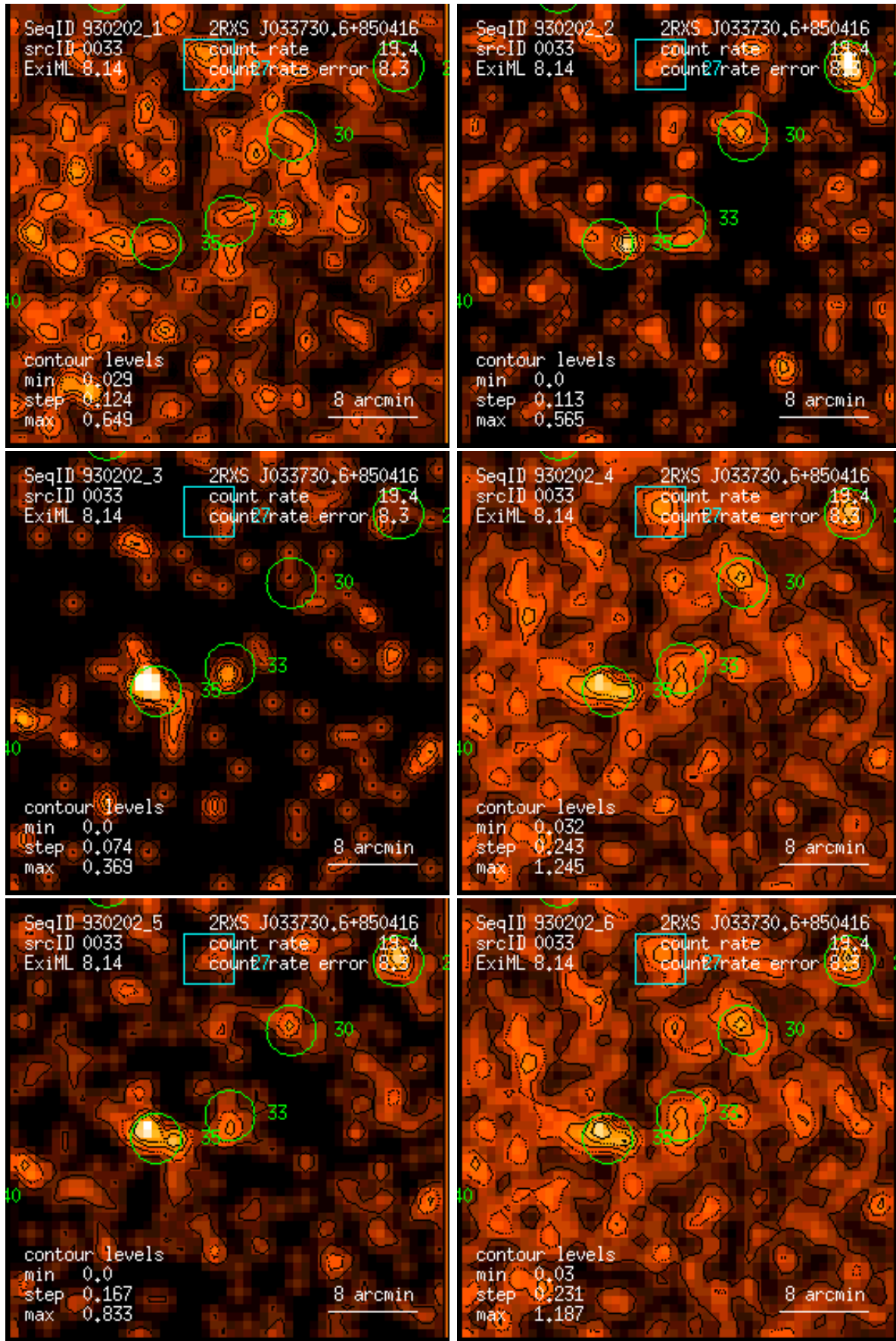
Figure 33: RASS 930202: detection 0033: band rate images, Gaussian filter: (1) PSPC channels 11 – 41, (2) 52 – 90, (3) 91 – 201, (4) 11 – 235, (5) 52 – 201, (6) 11 – 201. Broad band rates in counts/ks. Band rate contour levels in counts/ks/arcmin 2 .
