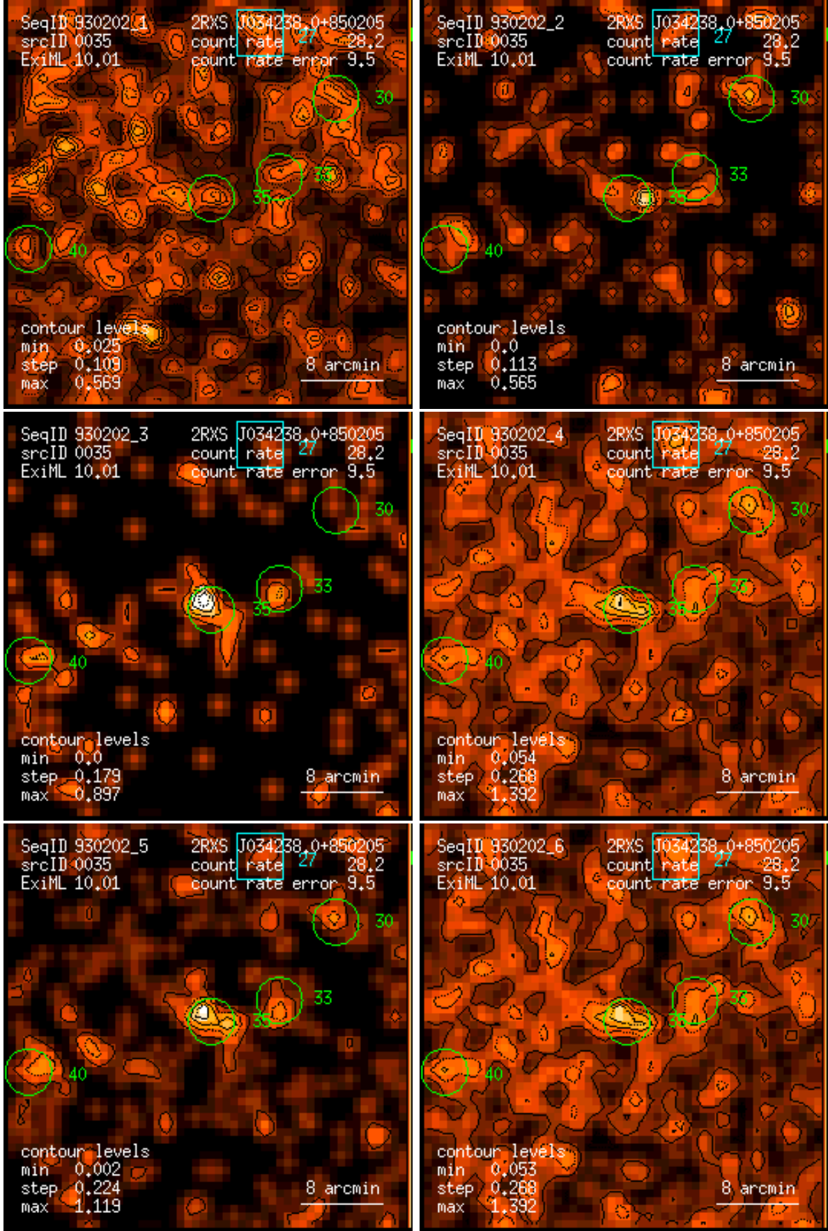
Figure 35: RASS 930202: detection 0035: band rate images, Gaussian filter: (1) PSPC channels 11 – 41, (2) 52 – 90, (3) 91 – 201, (4) 11 – 235, (5) 52 – 201, (6) 11 – 201. Broad band rates in counts/ks. Band rate contour levels in counts/ks/arcmin 2 .
