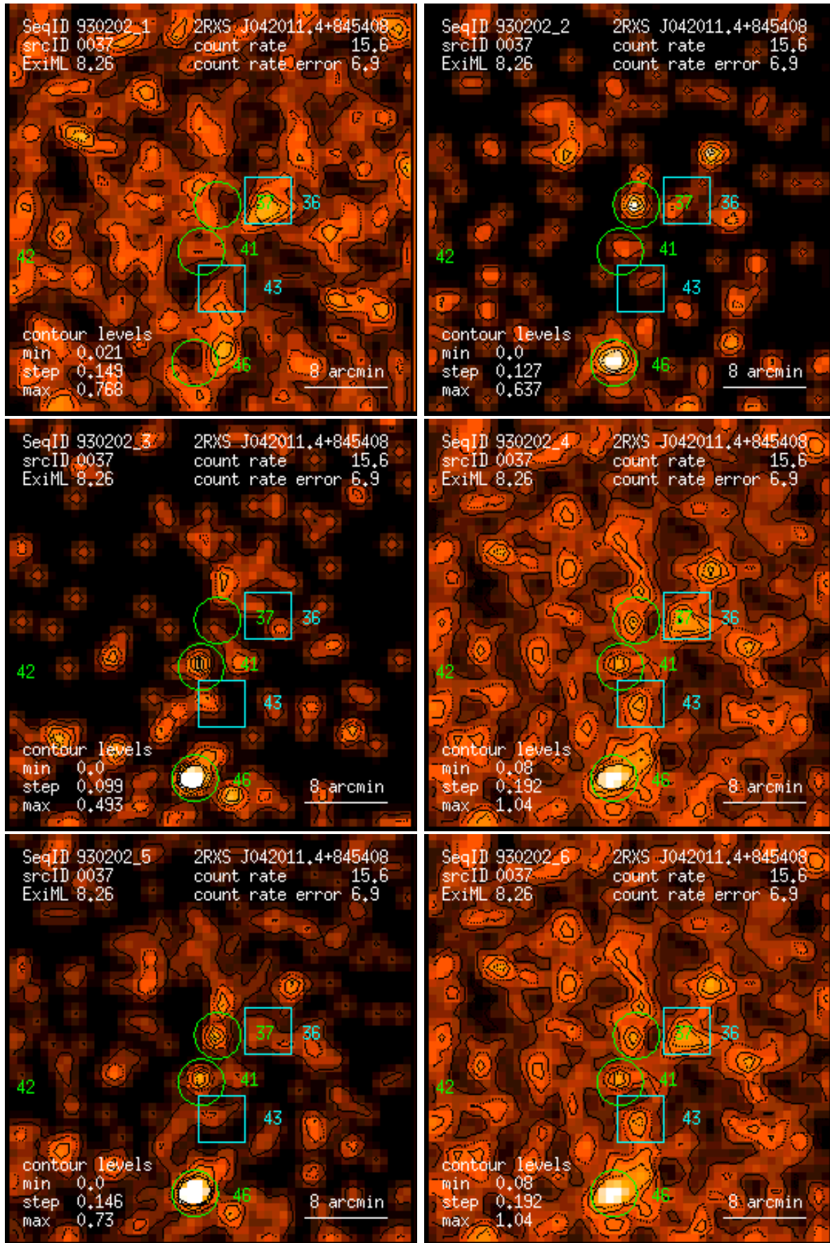
Figure 37: RASS 930202: detection 0037: band rate images, Gaussian filter: (1) PSPC channels 11 – 41, (2) 52 – 90, (3) 91 – 201, (4) 11 – 235, (5) 52 – 201, (6) 11 – 201. Broad band rates in counts/ks. Band rate contour levels in counts/ks/arcmin 2 .
