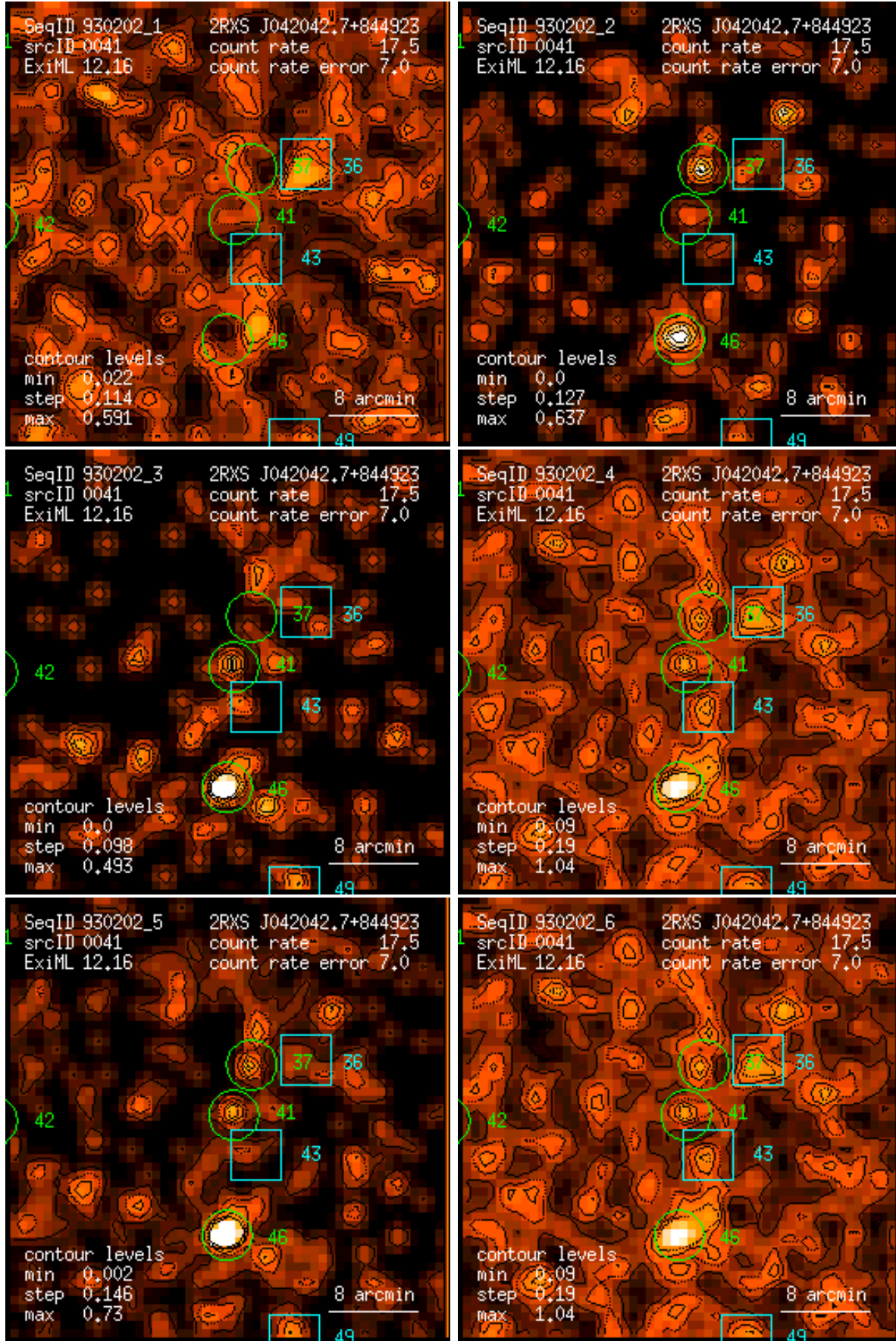
Figure 41: RASS 930202: detection 0041: band rate images, Gaussian filter: (1) PSPC channels 11 – 41, (2) 52 – 90, (3) 91 – 201, (4) 11 – 235, (5) 52 – 201, (6) 11 – 201. Broad band rates in counts/ks. Band rate contour levels in counts/ks/arcmin 2 .
