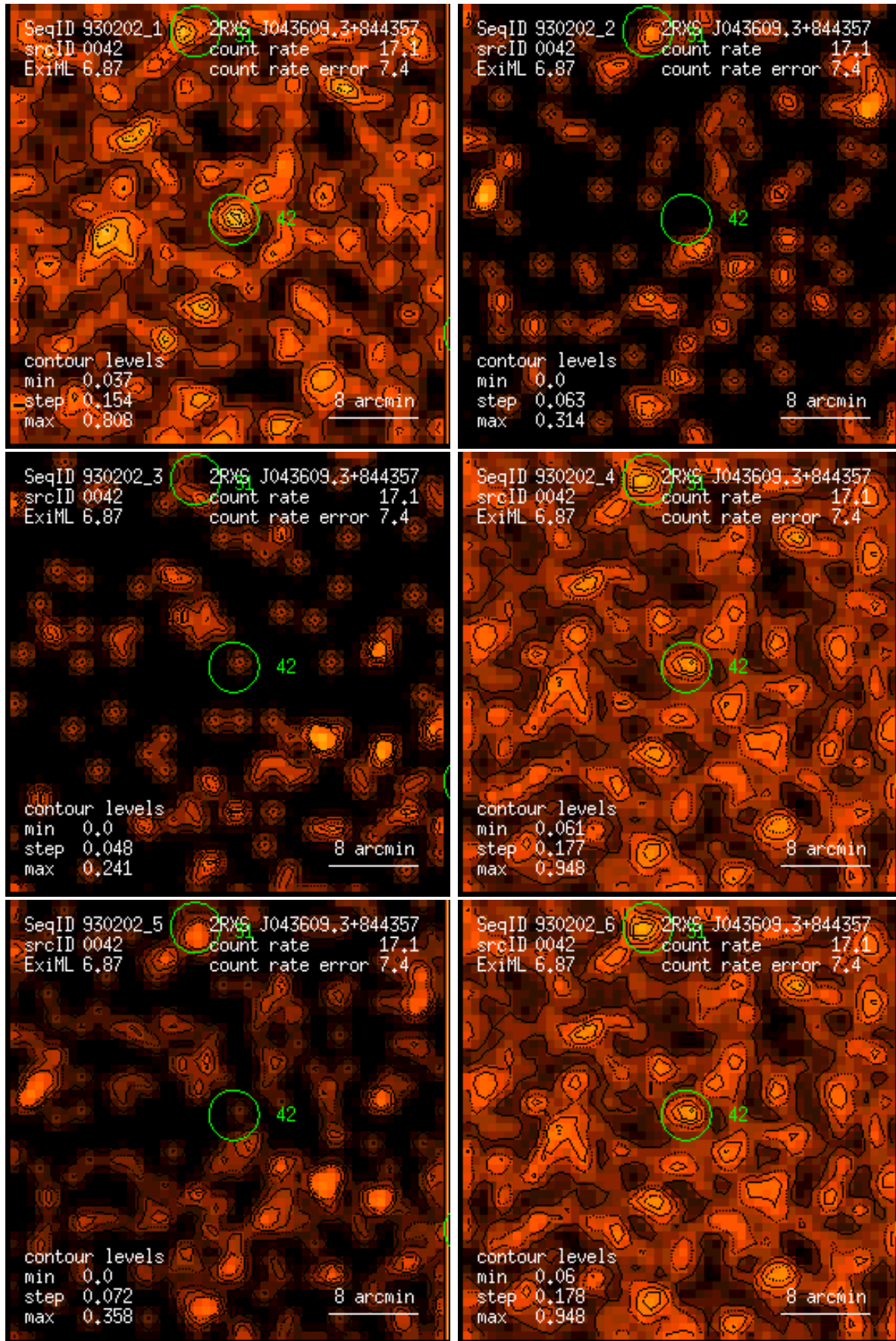
Figure 42: RASS 930202: detection 0042: band rate images, Gaussian filter: (1) PSPC channels 11 – 41, (2) 52 – 90, (3) 91 – 201, (4) 11 – 235, (5) 52 – 201, (6) 11 – 201. Broad band rates in counts/ks. Band rate contour levels in counts/ks/arcmin 2 .
