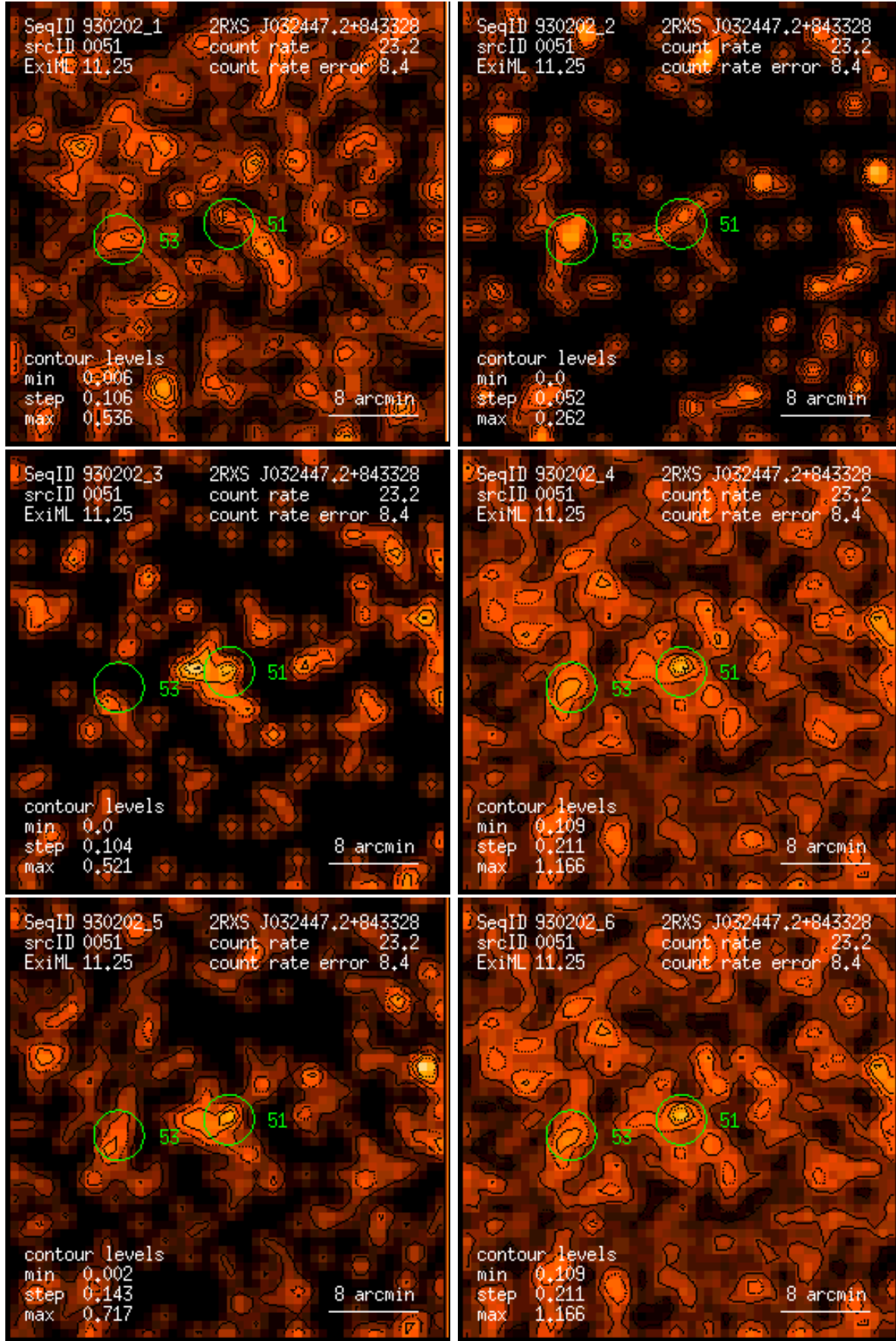
Figure 51: RASS 930202: detection 0051: band rate images, Gaussian filter: (1) PSPC channels 11 – 41, (2) 52 – 90, (3) 91 – 201, (4) 11 – 235, (5) 52 – 201, (6) 11 – 201. Broad band rates in counts/ks. Band rate contour levels in counts/ks/arcmin 2 .
