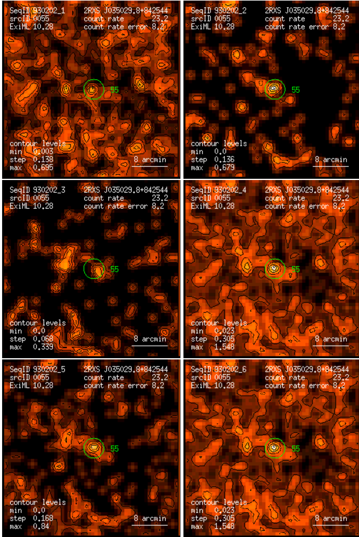
Figure 55: RASS 930202: detection 0055: band rate images, Gaussian filter: (1) PSPC channels 11 – 41, (2) 52 – 90, (3) 91 – 201, (4) 11 – 235, (5) 52 – 201, (6) 11 – 201. Broad band rates in counts/ks. Band rate contour levels in counts/ks/arcmin 2 .
