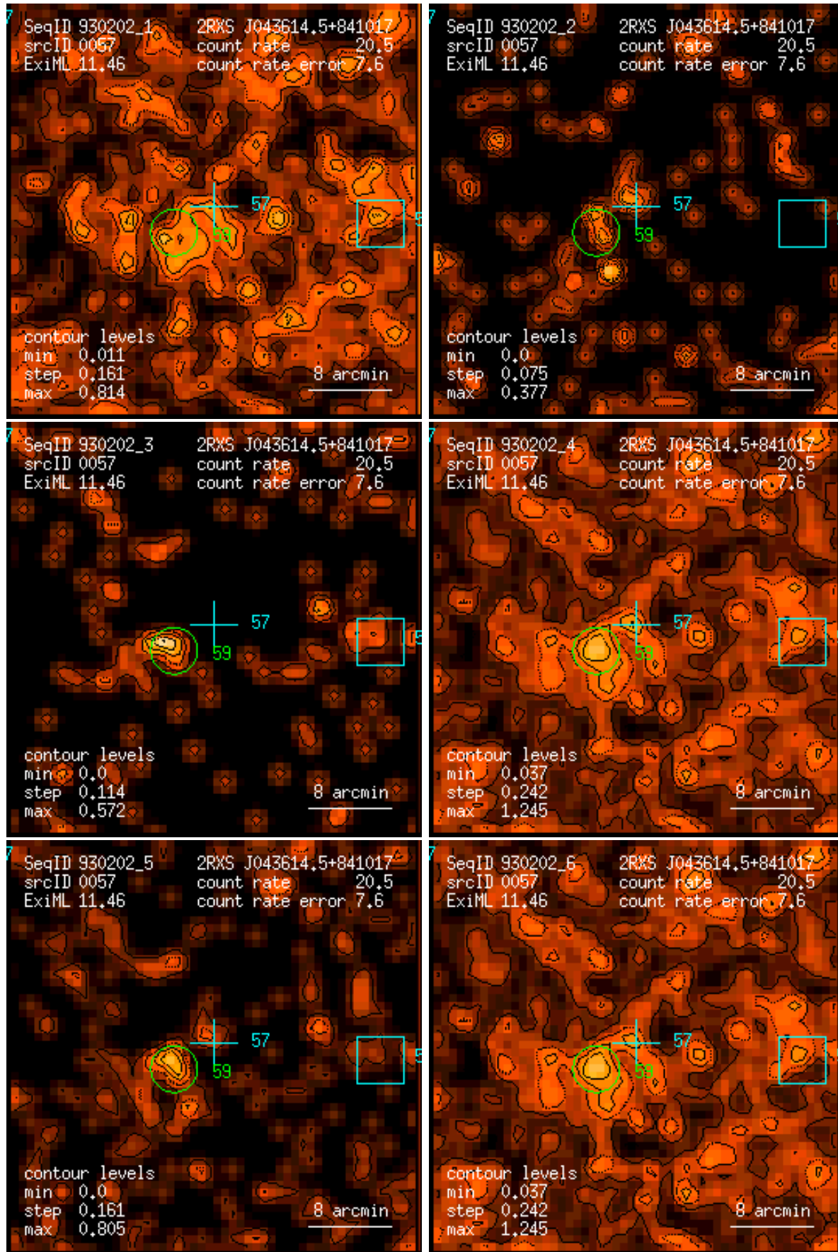
Figure 57: RASS 930202: detection 0057: band rate images, Gaussian filter: (1) PSPC channels 11 – 41, (2) 52 – 90, (3) 91 – 201, (4) 11 – 235, (5) 52 – 201, (6) 11 – 201. Broad band rates in counts/ks. Band rate contour levels in counts/ks/arcmin 2 .
