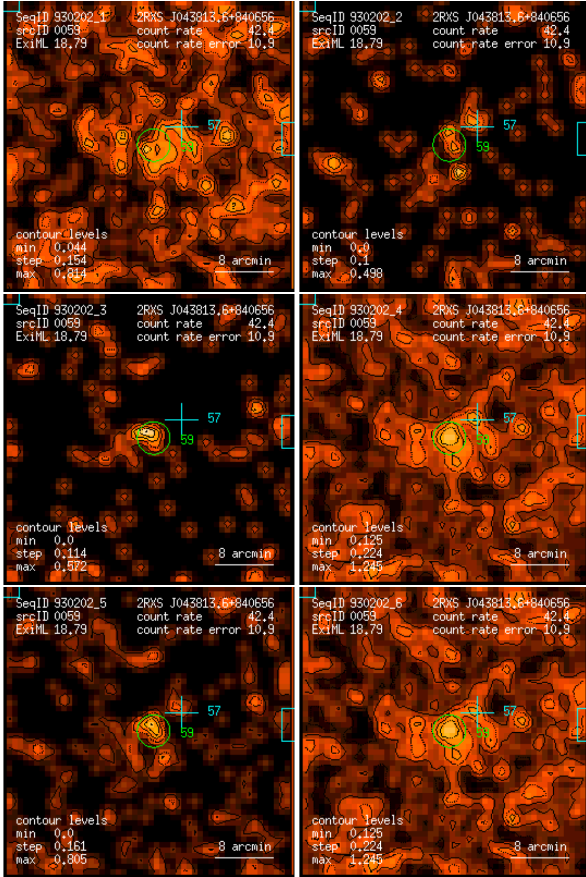
Figure 59: RASS 930202: detection 0059: band rate images, Gaussian filter: (1) PSPC channels 11 – 41, (2) 52 – 90, (3) 91 – 201, (4) 11 – 235, (5) 52 – 201, (6) 11 – 201. Broad band rates in counts/ks. Band rate contour levels in counts/ks/arcmin 2 .
