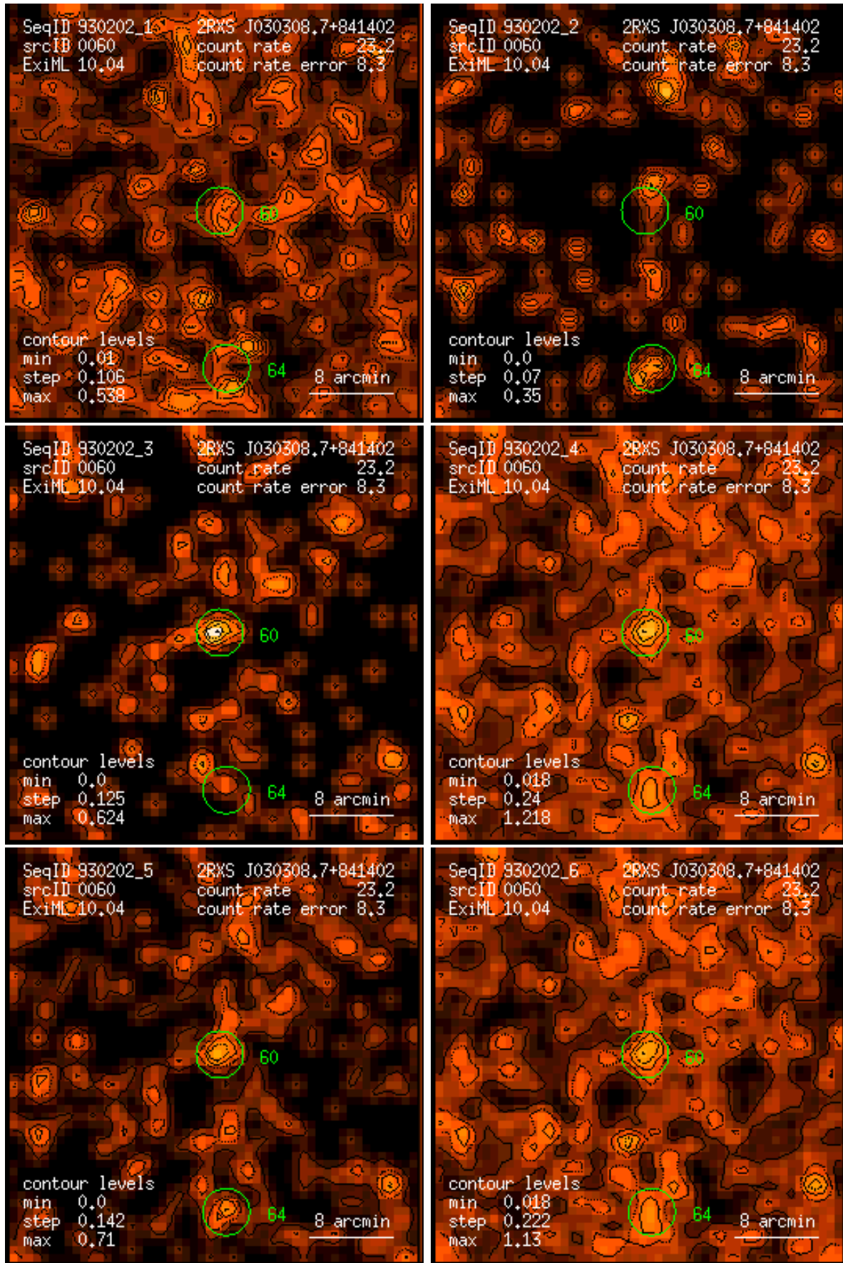
Figure 60: RASS 930202: detection 0060: band rate images, Gaussian filter: (1) PSPC channels 11 – 41, (2) 52 – 90, (3) 91 – 201, (4) 11 – 235, (5) 52 – 201, (6) 11 – 201. Broad band rates in counts/ks. Band rate contour levels in counts/ks/arcmin 2 .
