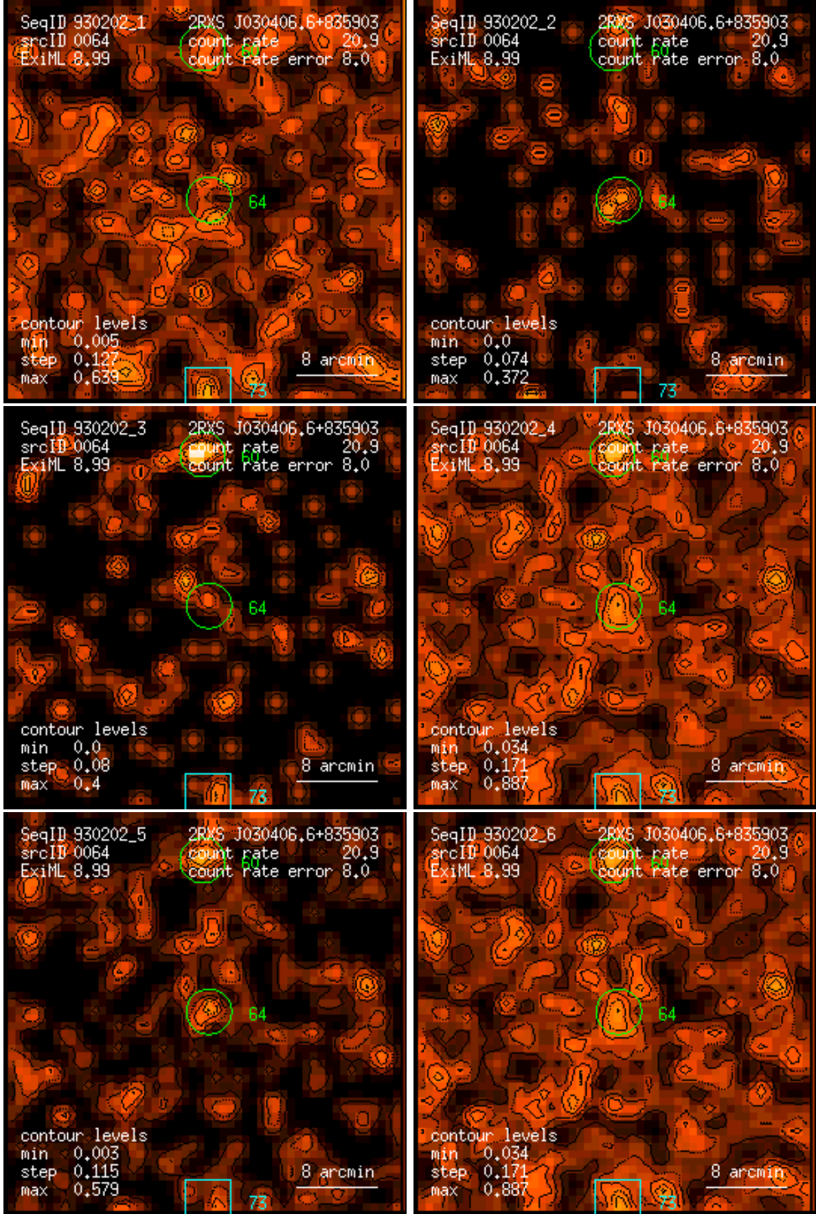
Figure 64: RASS 930202: detection 0064: band rate images, Gaussian filter: (1) PSPC channels 11 – 41, (2) 52 – 90, (3) 91 – 201, (4) 11 – 235, (5) 52 – 201, (6) 11 – 201. Broad band rates in counts/ks. Band rate contour levels in counts/ks/arcmin 2 .
