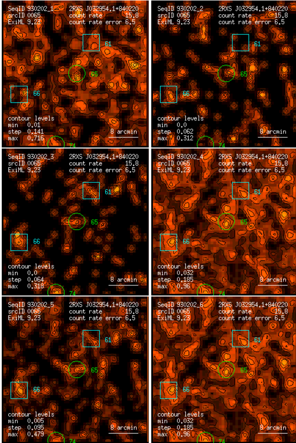
Figure 65: RASS 930202: detection 0065: band rate images, Gaussian filter: (1) PSPC channels 11 – 41, (2) 52 – 90, (3) 91 – 201, (4) 11 – 235, (5) 52 – 201, (6) 11 – 201. Broad band rates in counts/ks. Band rate contour levels in counts/ks/arcmin 2 .
