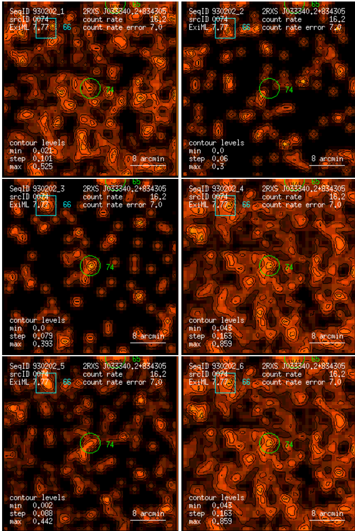
Figure 74: RASS 930202: detection 0074: band rate images, Gaussian filter: (1) PSPC channels 11 – 41, (2) 52 – 90, (3) 91 – 201, (4) 11 – 235, (5) 52 – 201, (6) 11 – 201. Broad band rates in counts/ks. Band rate contour levels in counts/ks/arcmin 2 .
