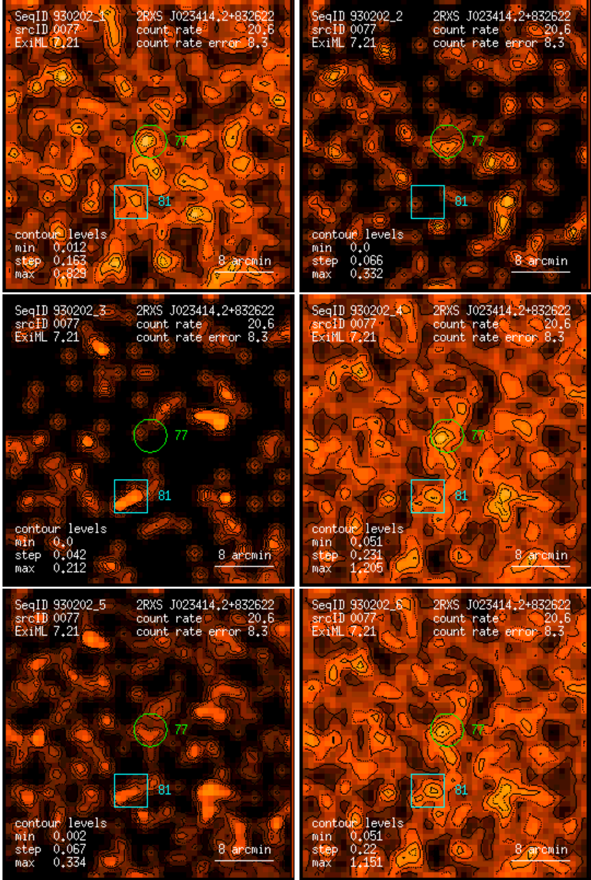
Figure 77: RASS 930202: detection 0077: band rate images, Gaussian filter: (1) PSPC channels 11 – 41, (2) 52 – 90, (3) 91 – 201, (4) 11 – 235, (5) 52 – 201, (6) 11 – 201. Broad band rates in counts/ks. Band rate contour levels in counts/ks/arcmin 2 .
