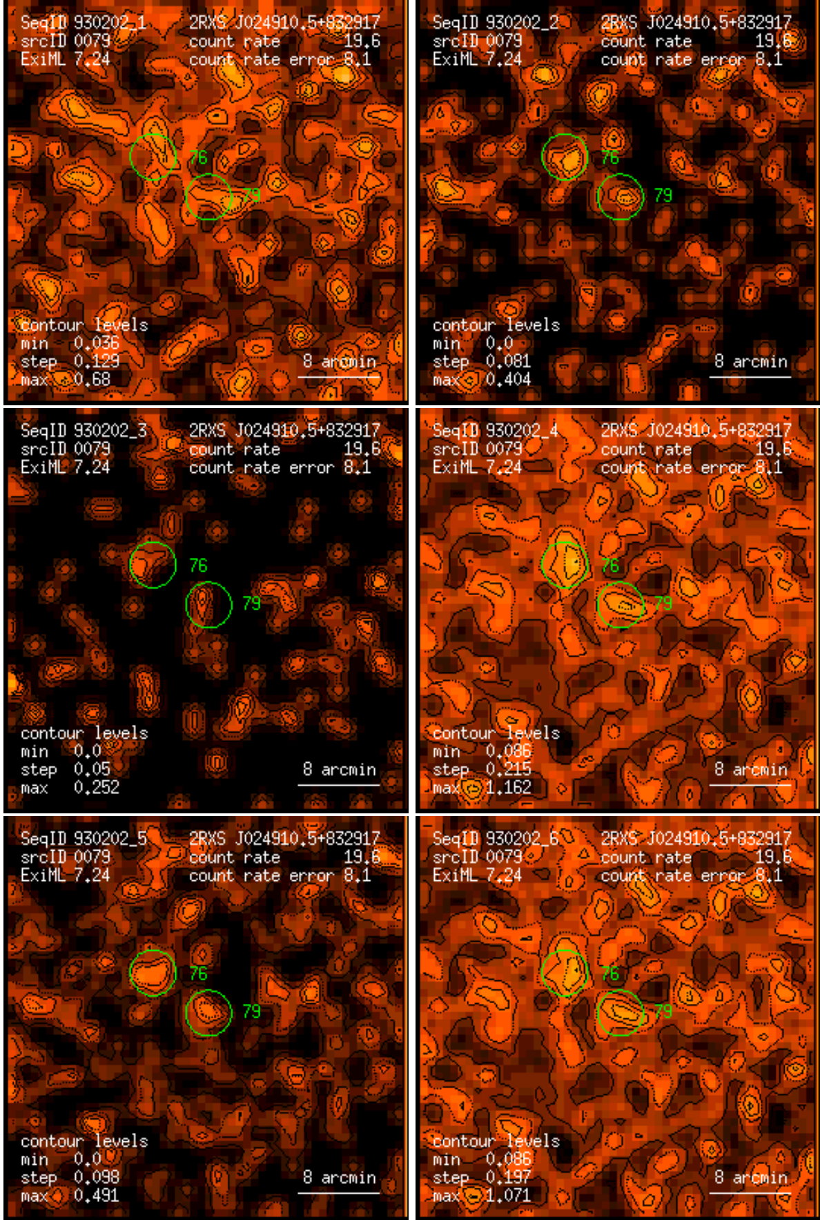
Figure 79: RASS 930202: detection 0079: band rate images, Gaussian filter: (1) PSPC channels 11 – 41, (2) 52 – 90, (3) 91 – 201, (4) 11 – 235, (5) 52 – 201, (6) 11 – 201. Broad band rates in counts/ks. Band rate contour levels in counts/ks/arcmin 2 .
