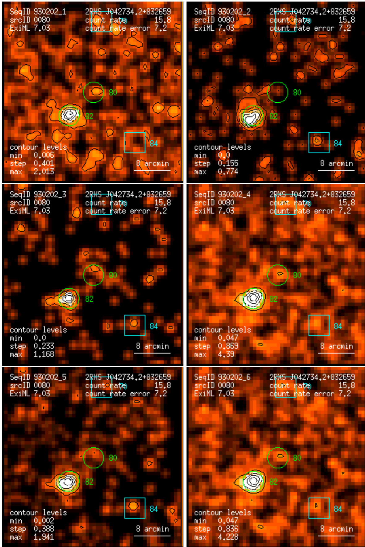
Figure 80: RASS 930202: detection 0080: band rate images, Gaussian filter: (1) PSPC channels 11 – 41, (2) 52 – 90, (3) 91 – 201, (4) 11 – 235, (5) 52 – 201, (6) 11 – 201. Broad band rates in counts/ks. Band rate contour levels in counts/ks/arcmin 2 .
