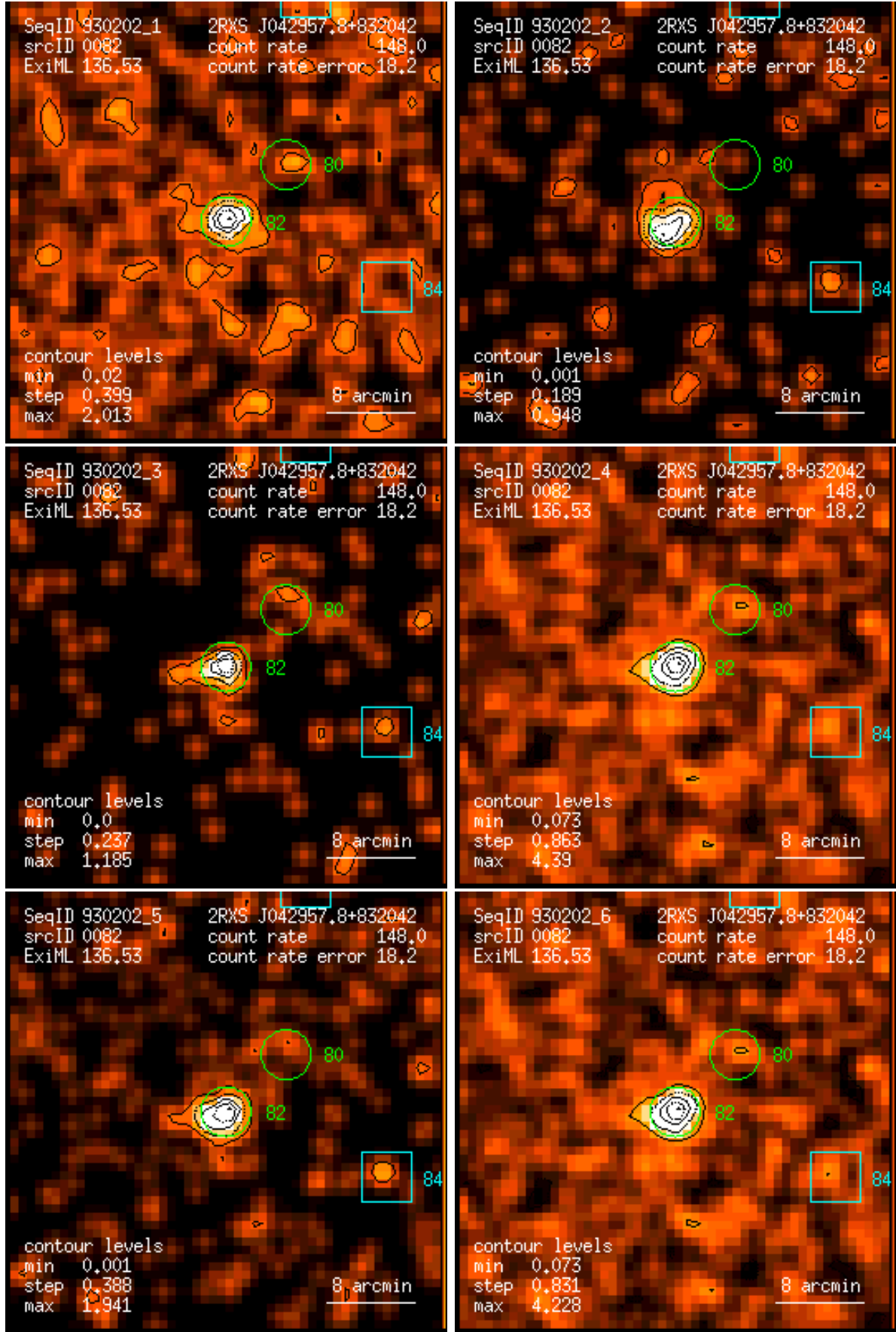
Figure 82: RASS 930202: detection 0082: band rate images, Gaussian filter: (1) PSPC channels 11 – 41, (2) 52 – 90, (3) 91 – 201, (4) 11 – 235, (5) 52 – 201, (6) 11 – 201. Broad band rates in counts/ks. Band rate contour levels in counts/ks/arcmin 2 .
