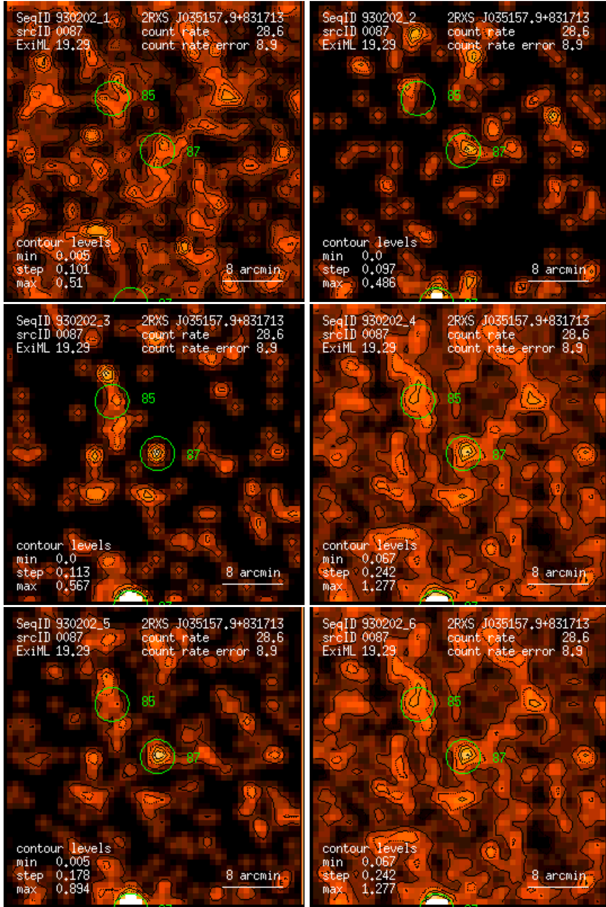
Figure 87: RASS 930202: detection 0087: band rate images, Gaussian filter: (1) PSPC channels 11 – 41, (2) 52 – 90, (3) 91 – 201, (4) 11 – 235, (5) 52 – 201, (6) 11 – 201. Broad band rates in counts/ks. Band rate contour levels in counts/ks/arcmin 2 .
