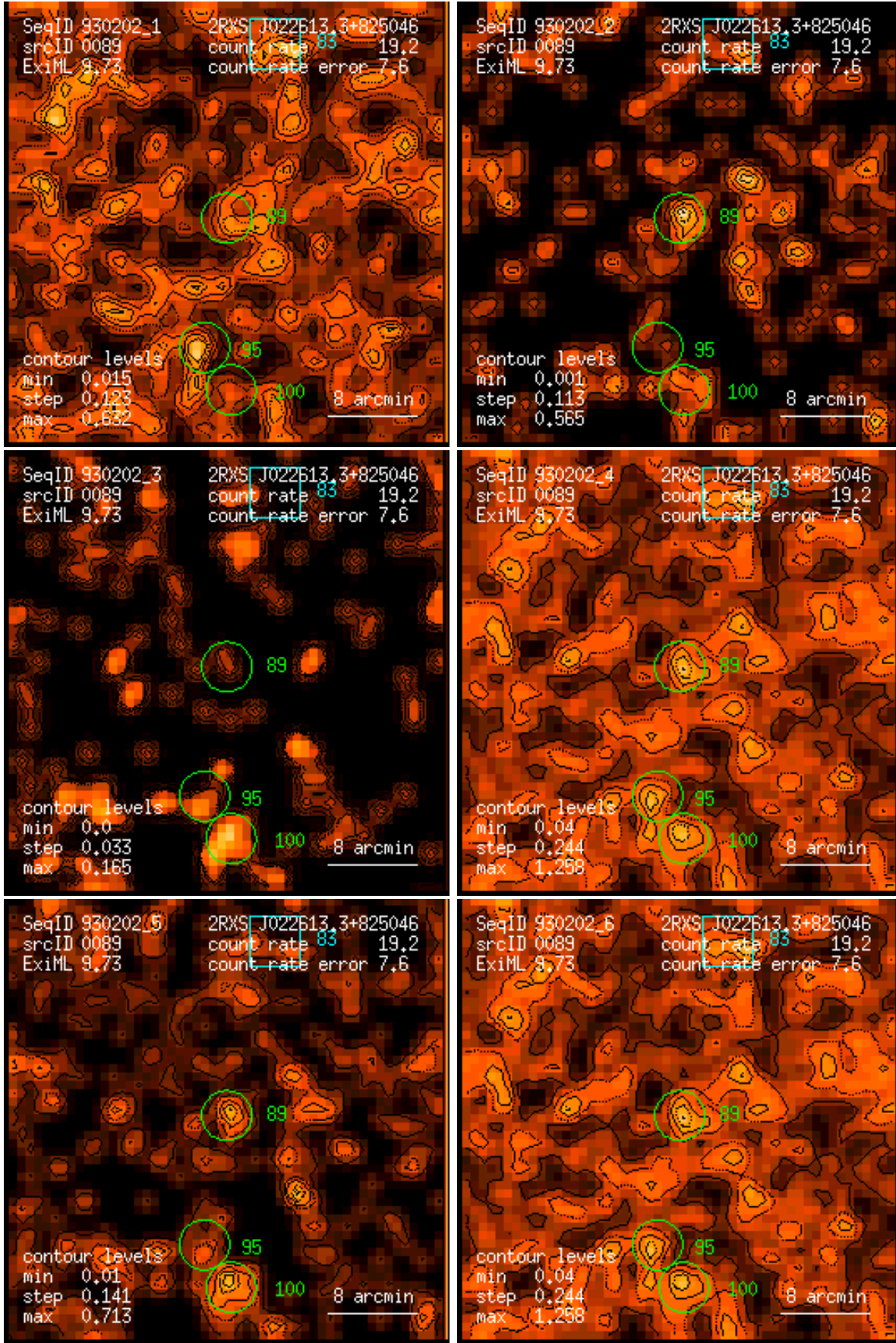
Figure 89: RASS 930202: detection 0089: band rate images, Gaussian filter: (1) PSPC channels 11 – 41, (2) 52 – 90, (3) 91 – 201, (4) 11 – 235, (5) 52 – 201, (6) 11 – 201. Broad band rates in counts/ks. Band rate contour levels in counts/ks/arcmin 2 .
