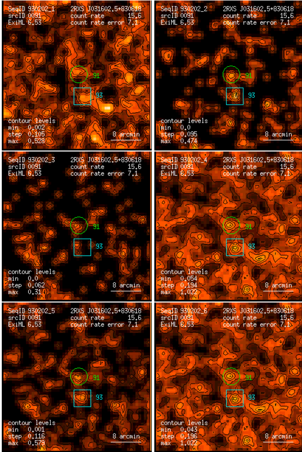
Figure 91: RASS 930202: detection 0091: band rate images, Gaussian filter: (1) PSPC channels 11 – 41, (2) 52 – 90, (3) 91 – 201, (4) 11 – 235, (5) 52 – 201, (6) 11 – 201. Broad band rates in counts/ks. Band rate contour levels in counts/ks/arcmin 2 .
