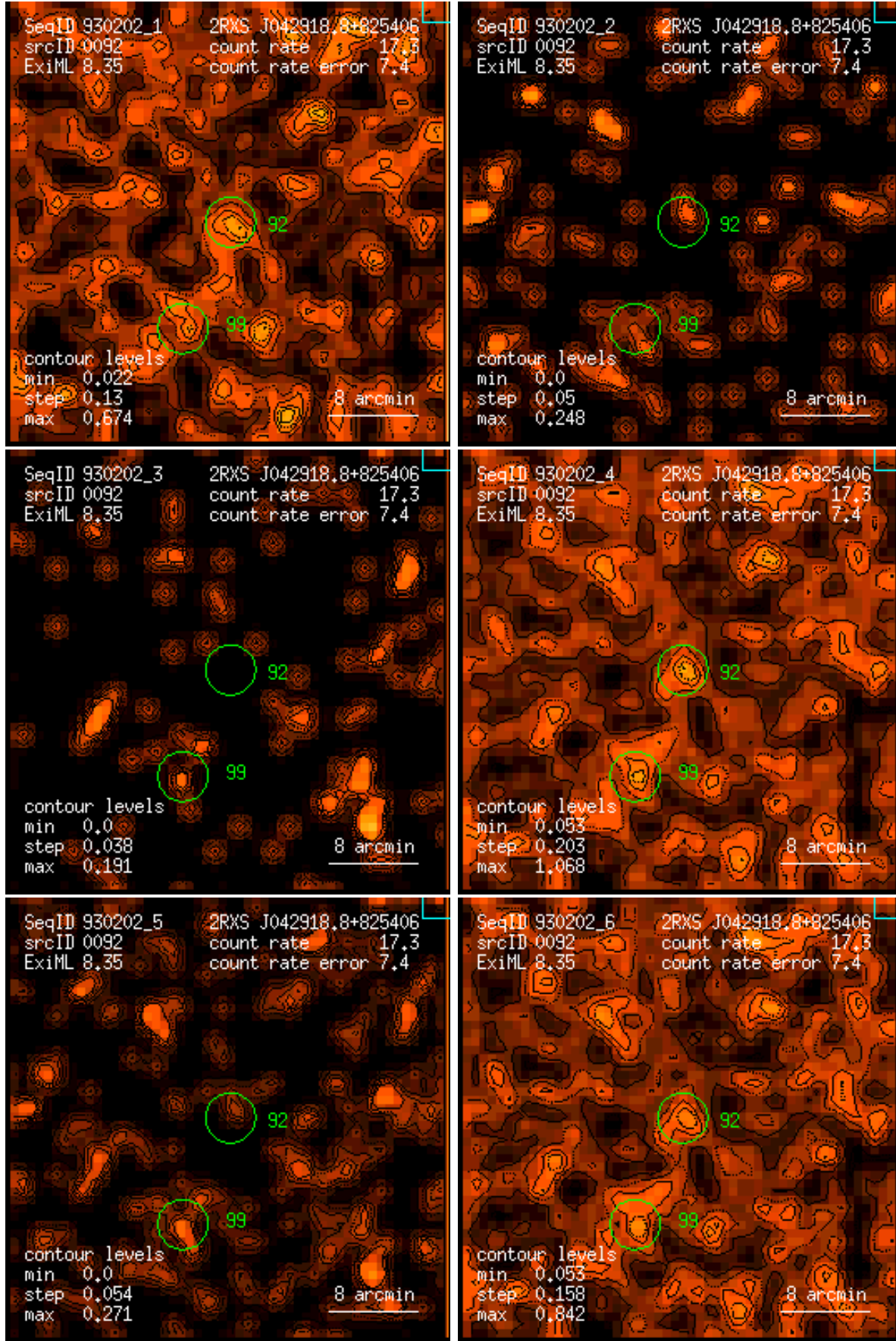
Figure 92: RASS 930202: detection 0092: band rate images, Gaussian filter: (1) PSPC channels 11 – 41, (2) 52 – 90, (3) 91 – 201, (4) 11 – 235, (5) 52 – 201, (6) 11 – 201. Broad band rates in counts/ks. Band rate contour levels in counts/ks/arcmin 2 .
