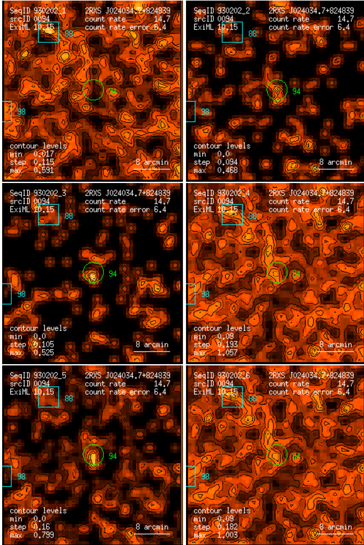
Figure 94: RASS 930202: detection 0094: band rate images, Gaussian filter: (1) PSPC channels 11 – 41, (2) 52 – 90, (3) 91 – 201, (4) 11 – 235, (5) 52 – 201, (6) 11 – 201. Broad band rates in counts/ks. Band rate contour levels in counts/ks/arcmin 2 .
