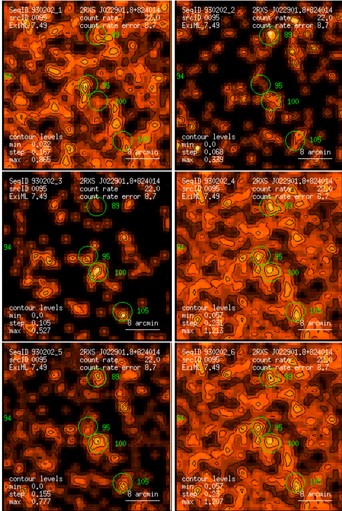
Figure 95: RASS 930202: detection 0095: band rate images, Gaussian filter: (1) PSPC channels 11 – 41, (2) 52 – 90, (3) 91 – 201, (4) 11 – 235, (5) 52 – 201, (6) 11 – 201. Broad band rates in counts/ks. Band rate contour levels in counts/ks/arcmin 2 .
