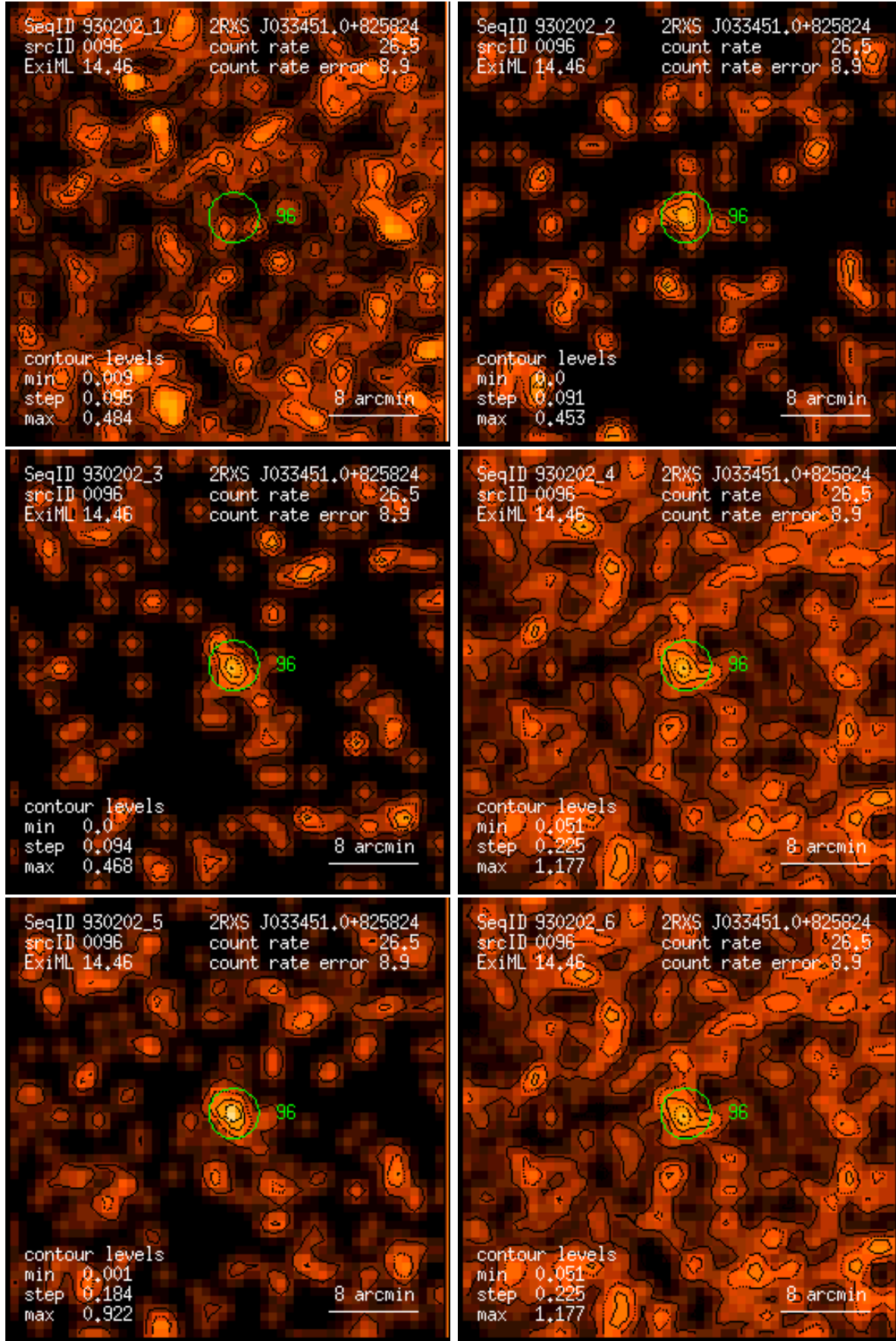
Figure 96: RASS 930202: detection 0096: band rate images, Gaussian filter: (1) PSPC channels 11 – 41, (2) 52 – 90, (3) 91 – 201, (4) 11 – 235, (5) 52 – 201, (6) 11 – 201. Broad band rates in counts/ks. Band rate contour levels in counts/ks/arcmin 2 .
