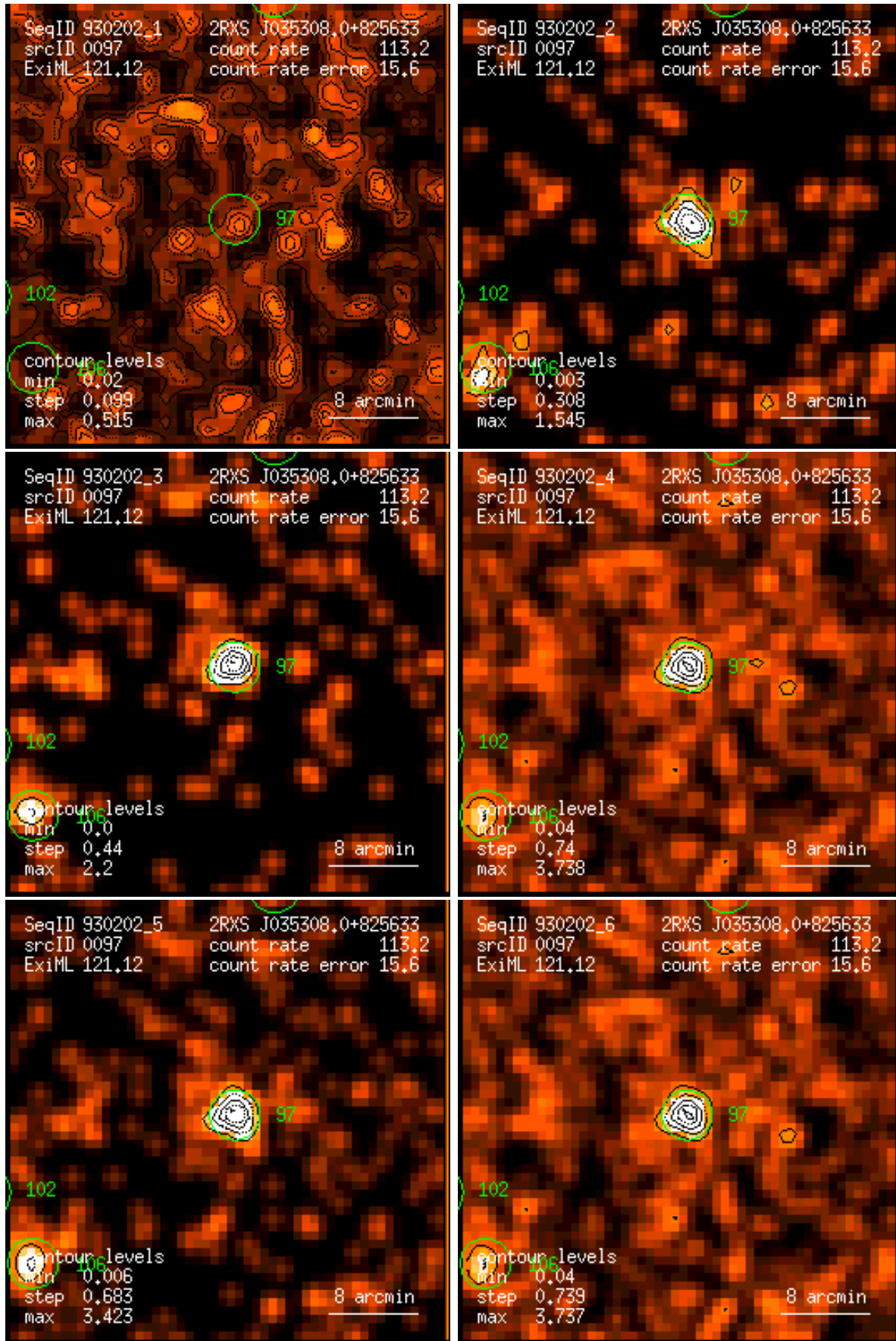
Figure 97: RASS 930202: detection 0097: band rate images, Gaussian filter: (1) PSPC channels 11 – 41, (2) 52 – 90, (3) 91 – 201, (4) 11 – 235, (5) 52 – 201, (6) 11 – 201. Broad band rates in counts/ks. Band rate contour levels in counts/ks/arcmin 2 .
