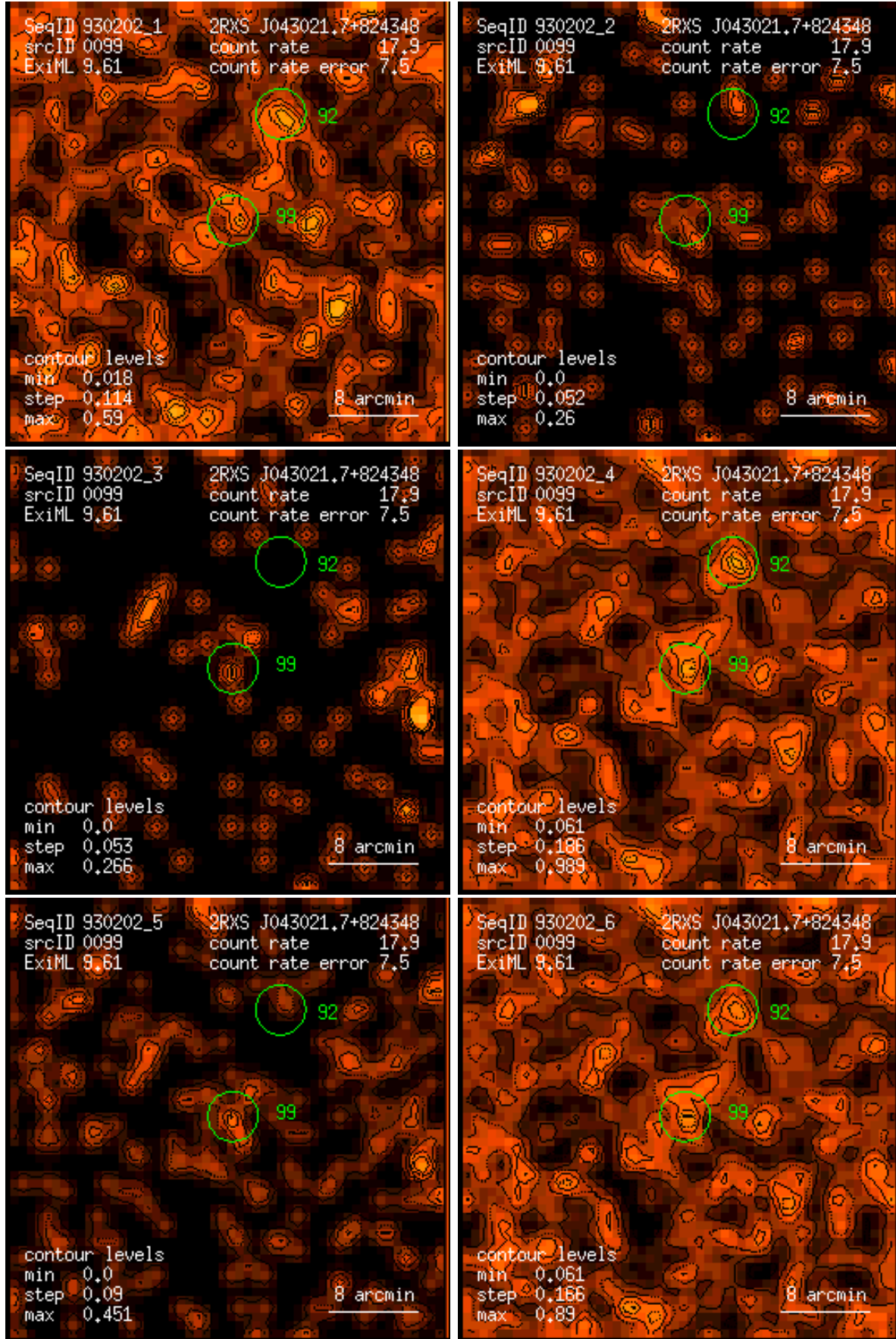
Figure 99: RASS 930202: detection 0099: band rate images, Gaussian filter: (1) PSPC channels 11 – 41, (2) 52 – 90, (3) 91 – 201, (4) 11 – 235, (5) 52 – 201, (6) 11 – 201. Broad band rates in counts/ks. Band rate contour levels in counts/ks/arcmin 2 .
