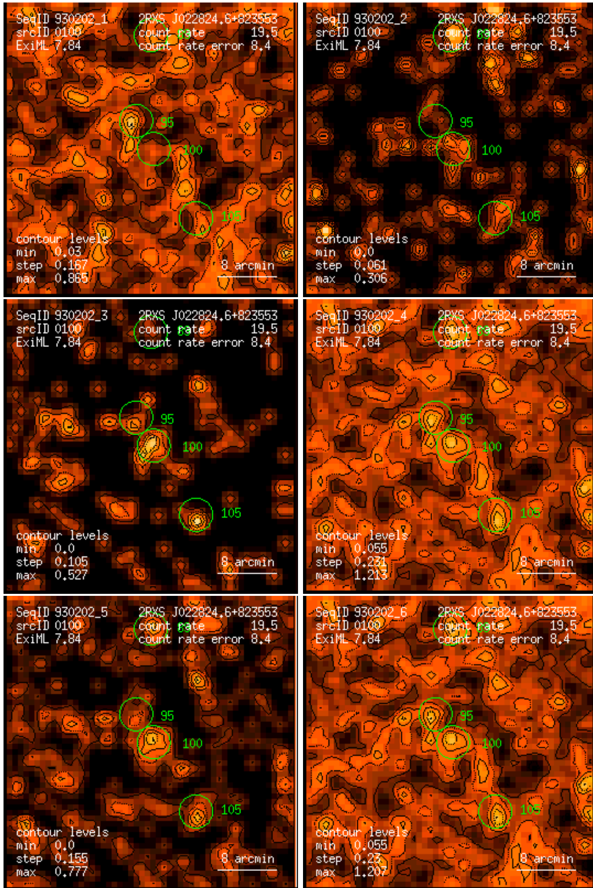
Figure 100: RASS 930202: detection 0100: band rate images, Gaussian filter: (1) PSPC channels 11 – 41, (2) 52 – 90, (3) 91 – 201, (4) 11 – 235, (5) 52 – 201, (6) 11 – 201. Broad band rates in counts/ks. Band rate contour levels in counts/ks/arcmin 2 .
