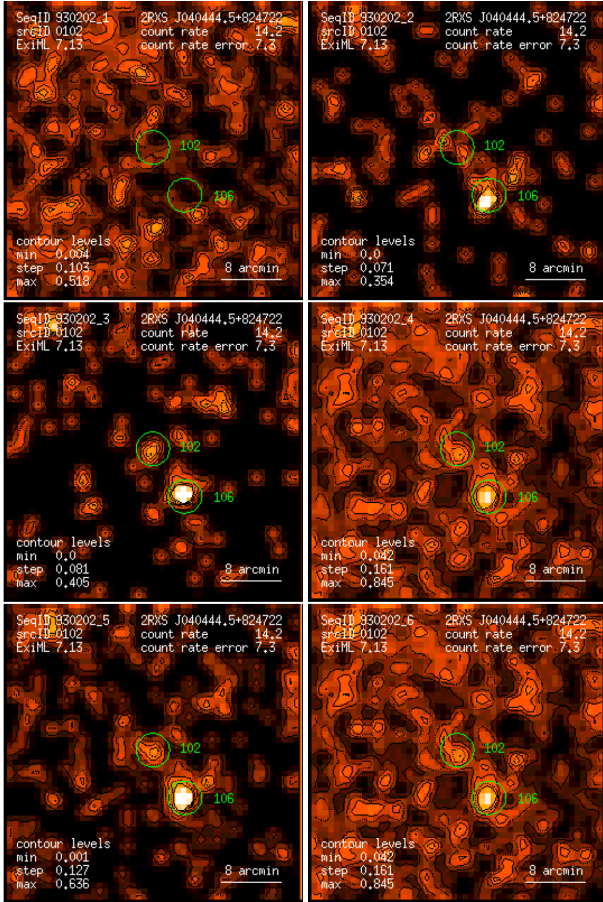
Figure 102: RASS 930202: detection 0102: band rate images, Gaussian filter: (1) PSPC channels 11 – 41, (2) 52 – 90, (3) 91 – 201, (4) 11 – 235, (5) 52 – 201, (6) 11 – 201. Broad band rates in counts/ks. Band rate contour levels in counts/ks/arcmin 2 .
