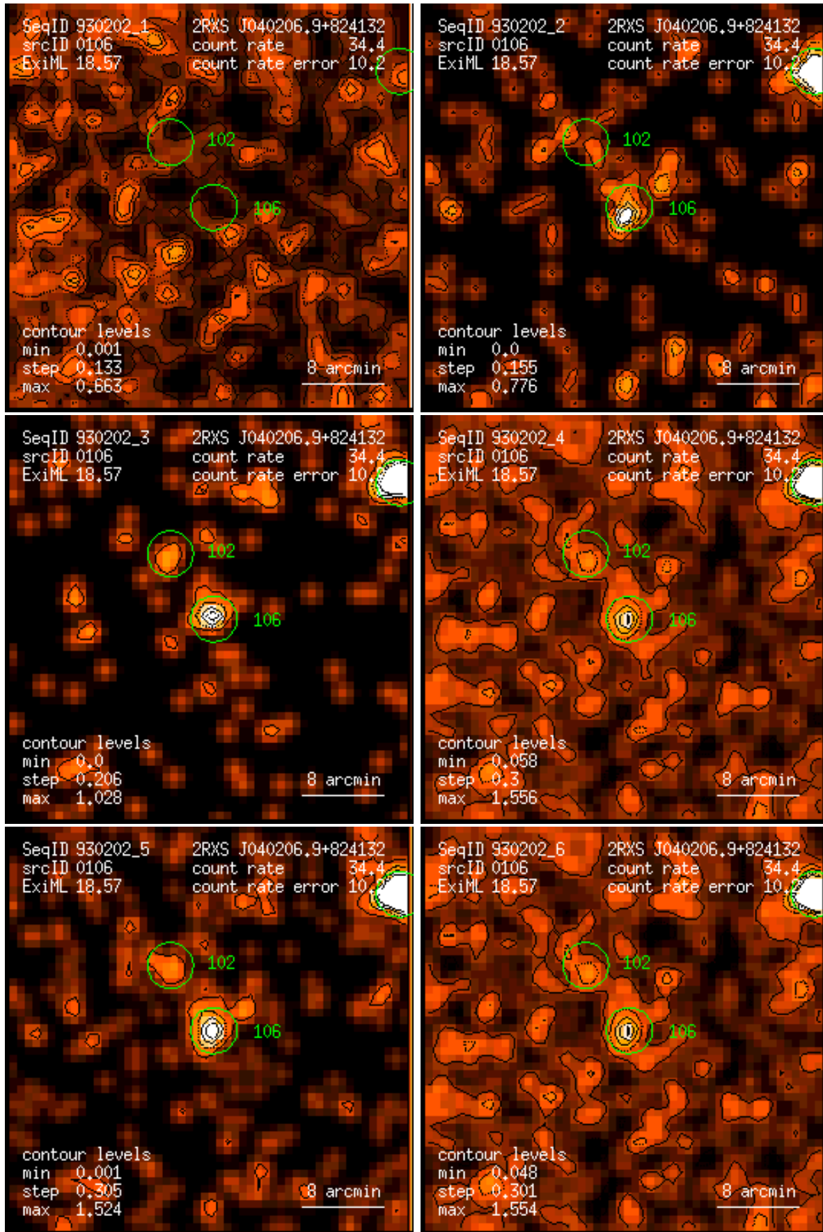
Figure 106: RASS 930202: detection 0106: band rate images, Gaussian filter: (1) PSPC channels 11 – 41, (2) 52 – 90, (3) 91 – 201, (4) 11 – 235, (5) 52 – 201, (6) 11 – 201. Broad band rates in counts/ks. Band rate contour levels in counts/ks/arcmin 2 .
