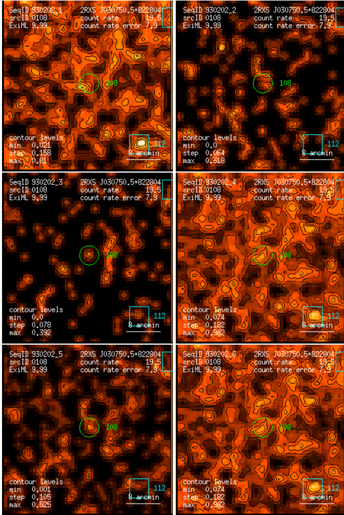
Figure 108: RASS 930202: detection 0108: band rate images, Gaussian filter: (1) PSPC channels 11 – 41, (2) 52 – 90, (3) 91 – 201, (4) 11 – 235, (5) 52 – 201, (6) 11 – 201. Broad band rates in counts/ks. Band rate contour levels in counts/ks/arcmin 2 .
