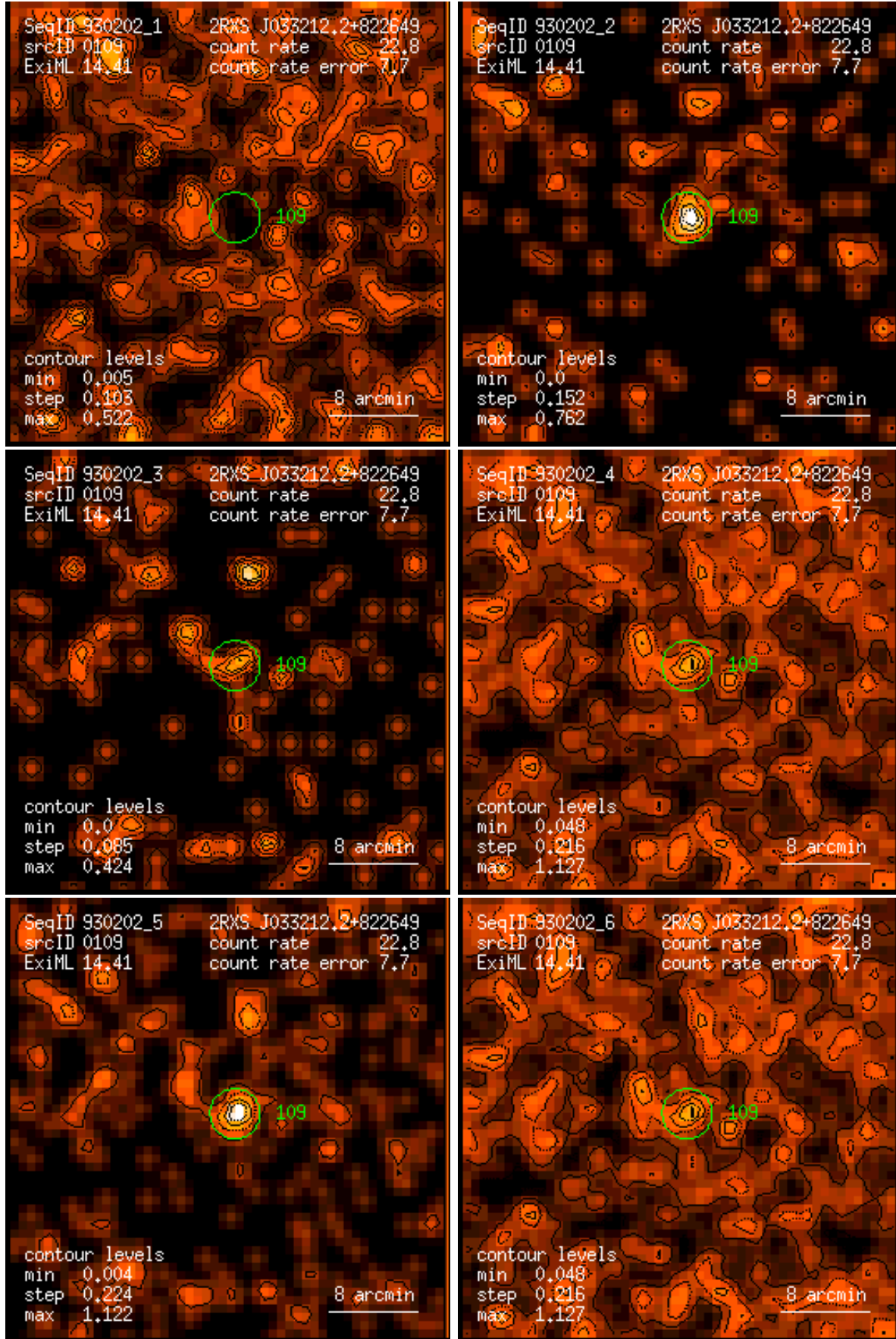
Figure 109: RASS 930202: detection 0109: band rate images, Gaussian filter: (1) PSPC channels 11 – 41, (2) 52 – 90, (3) 91 – 201, (4) 11 – 235, (5) 52 – 201, (6) 11 – 201. Broad band rates in counts/ks. Band rate contour levels in counts/ks/arcmin 2 .
