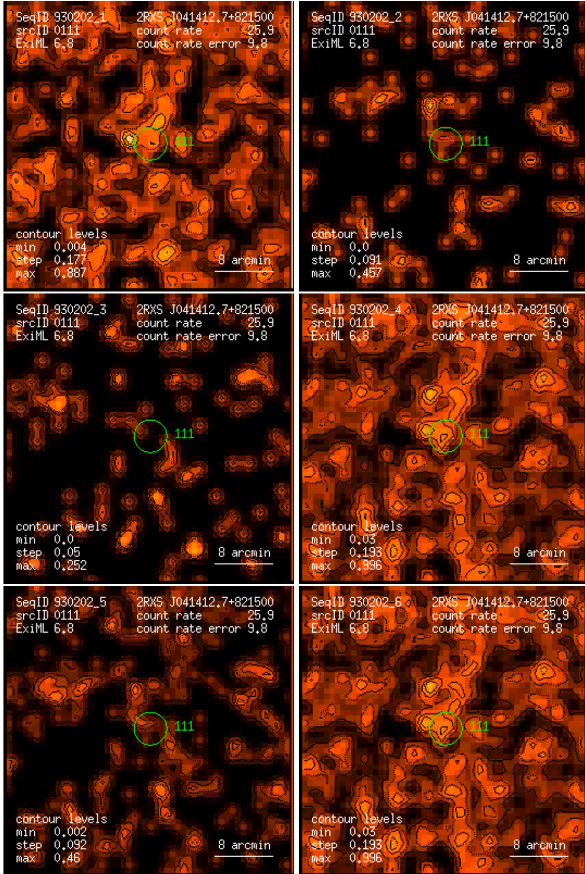
Figure 111: RASS 930202: detection 0111: band rate images, Gaussian filter: (1) PSPC channels 11 – 41, (2) 52 – 90, (3) 91 – 201, (4) 11 – 235, (5) 52 – 201, (6) 11 – 201. Broad band rates in counts/ks. Band rate contour levels in counts/ks/arcmin 2 .
