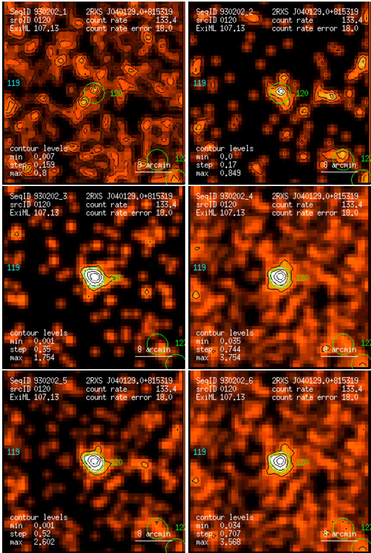
Figure 120: RASS 930202: detection 0120: band rate images, Gaussian filter: (1) PSPC channels 11 – 41, (2) 52 – 90, (3) 91 – 201, (4) 11 – 235, (5) 52 – 201, (6) 11 – 201. Broad band rates in counts/ks. Band rate contour levels in counts/ks/arcmin 2 .
