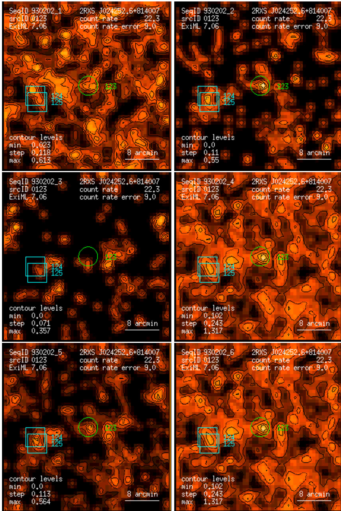
Figure 123: RASS 930202: detection 0123: band rate images, Gaussian filter: (1) PSPC channels 11 – 41, (2) 52 – 90, (3) 91 – 201, (4) 11 – 235, (5) 52 – 201, (6) 11 – 201. Broad band rates in counts/ks. Band rate contour levels in counts/ks/arcmin 2 .
