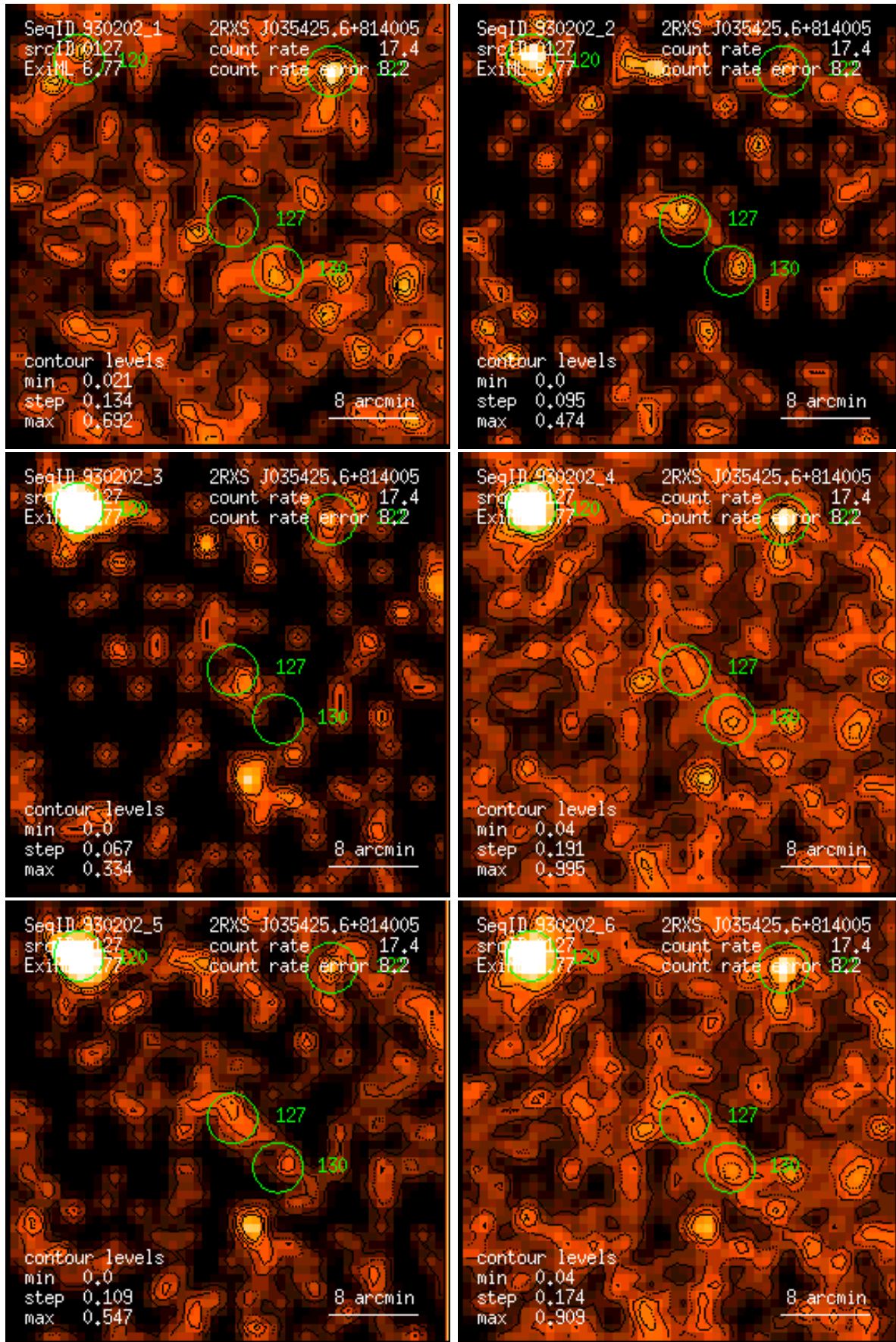
Figure 127: RASS 930202: detection 0127: band rate images, Gaussian filter: (1) PSPC channels 11 – 41, (2) 52 – 90, (3) 91 – 201, (4) 11 – 235, (5) 52 – 201, (6) 11 – 201. Broad band rates in counts/ks. Band rate contour levels in counts/ks/arcmin 2 .
