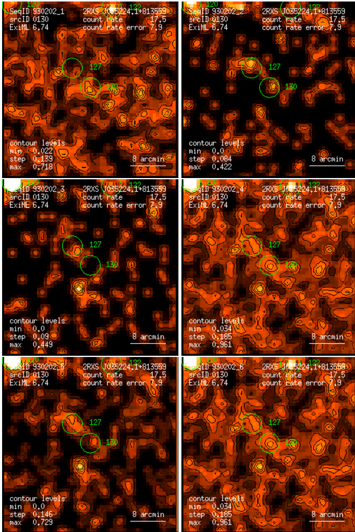
Figure 130: RASS 930202: detection 0130: band rate images, Gaussian filter: (1) PSPC channels 11 – 41, (2) 52 – 90, (3) 91 – 201, (4) 11 – 235, (5) 52 – 201, (6) 11 – 201. Broad band rates in counts/ks. Band rate contour levels in counts/ks/arcmin 2 .
