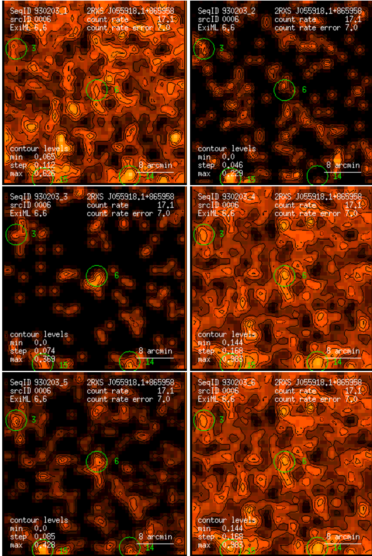
Figure 6: RASS 930203: detection 0006: band rate images, Gaussian filter: (1) PSPC channels 11 – 41, (2) 52 – 90, (3) 91 – 201, (4) 11 – 235, (5) 52 – 201, (6) 11 – 201. Broad band rates in counts/ks. Band rate contour levels in counts/ks/arcmin 2 .
