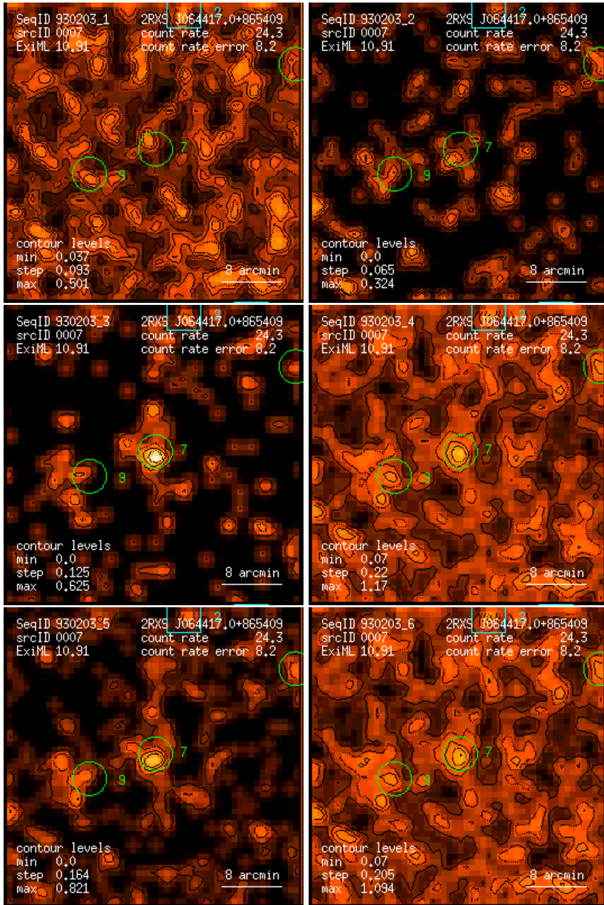
Figure 7: RASS 930203: detection 0007: band rate images, Gaussian filter: (1) PSPC channels 11 – 41, (2) 52 – 90, (3) 91 – 201, (4) 11 – 235, (5) 52 – 201, (6) 11 – 201. Broad band rates in counts/ks. Band rate contour levels in counts/ks/arcmin 2 .
