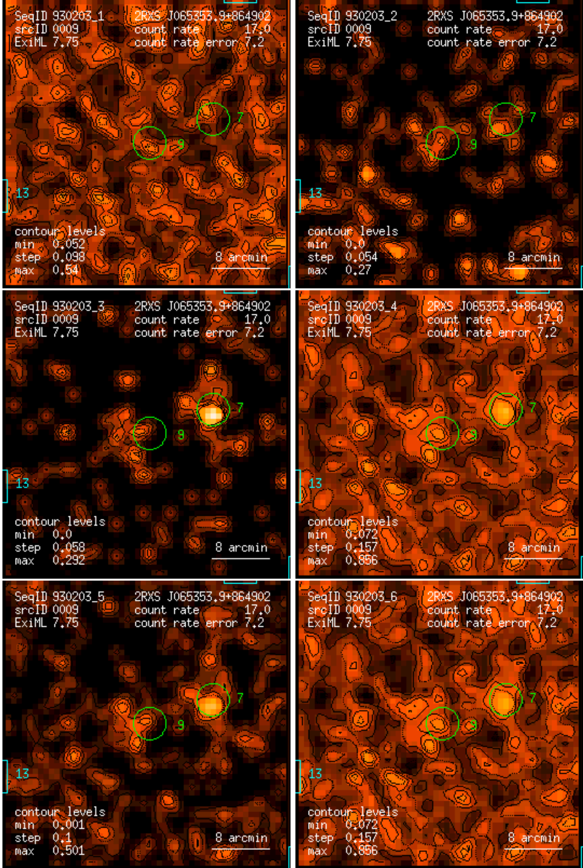
Figure 9: RASS 930203: detection 0009: band rate images, Gaussian filter: (1) PSPC channels 11 – 41, (2) 52 – 90, (3) 91 – 201, (4) 11 – 235, (5) 52 – 201, (6) 11 – 201. Broad band rates in counts/ks. Band rate contour levels in counts/ks/arcmin 2 .
