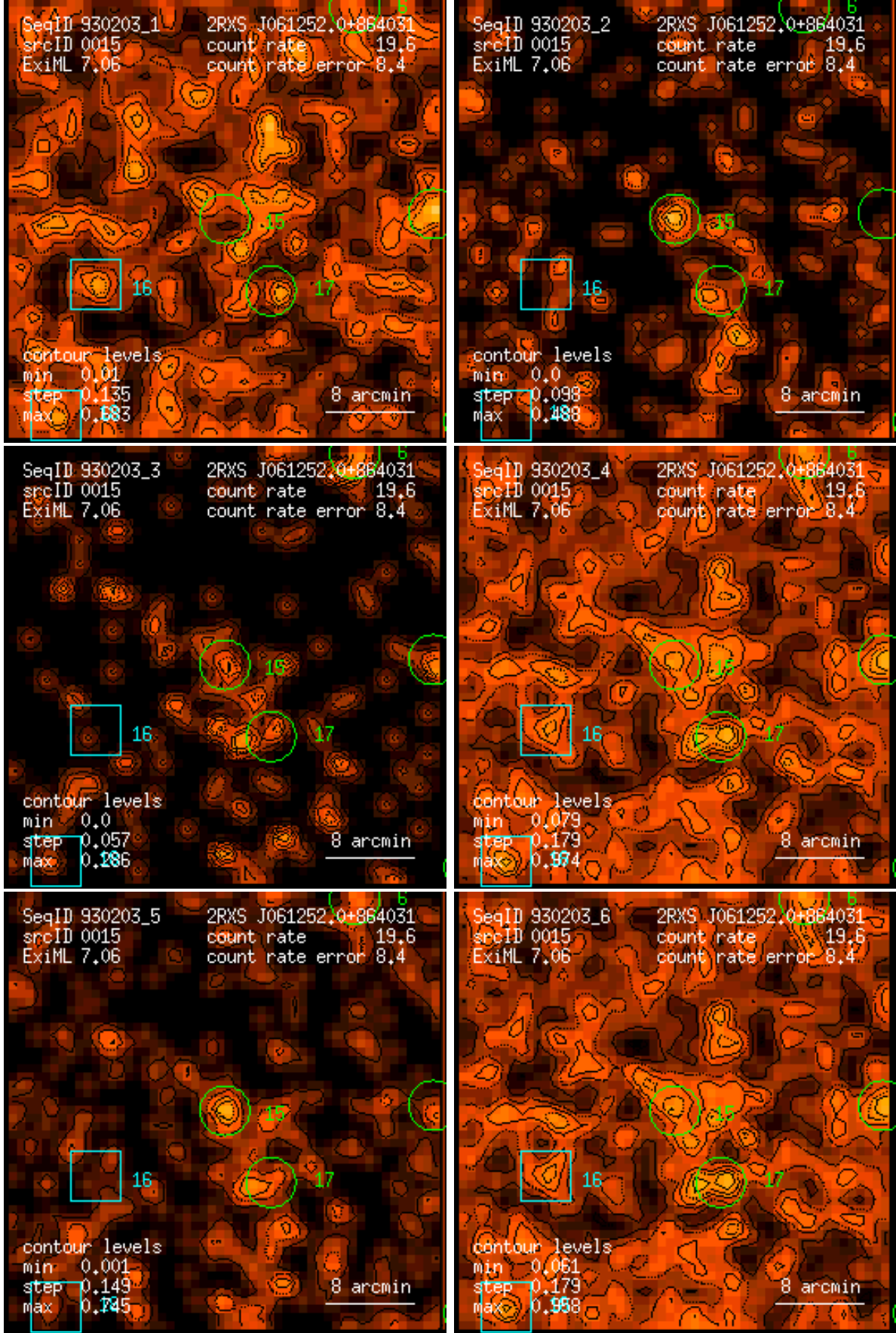
Figure 15: RASS 930203: detection 0015: band rate images, Gaussian filter: (1) PSPC channels 11 – 41, (2) 52 – 90, (3) 91 – 201, (4) 11 – 235, (5) 52 – 201, (6) 11 – 201. Broad band rates in counts/ks. Band rate contour levels in counts/ks/arcmin 2 .
